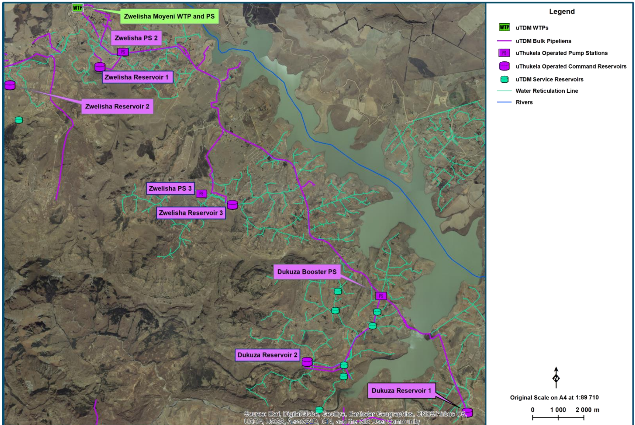
Figure 13.49 Zwelisha Moyeni WTP Supply System Layout NGI 2014; Umgeni Water 2020)
