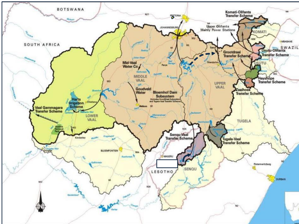
Figure 13.18 The Thukela-Vaal Transfer Scheme in the Vaal River System (DWS 2018: Slide 6).
