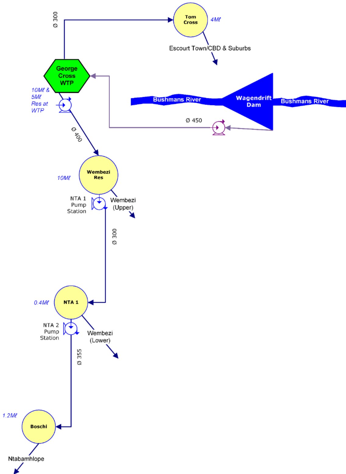
Figure 13.65 George Cross WTP Supply System Schematic (not to scale; uTDM Infrastructure)
