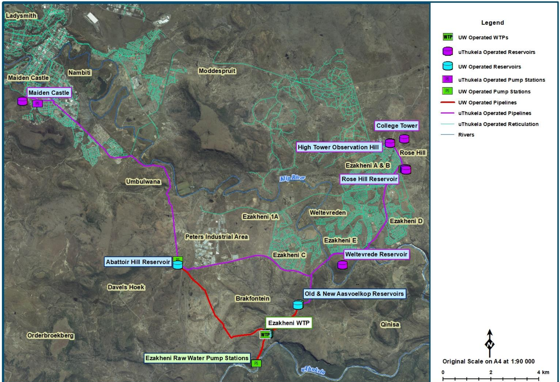
Figure 13.24 Ezakheni WTP Supply System layout (NGI 2014; Umgeni Water 2019).
