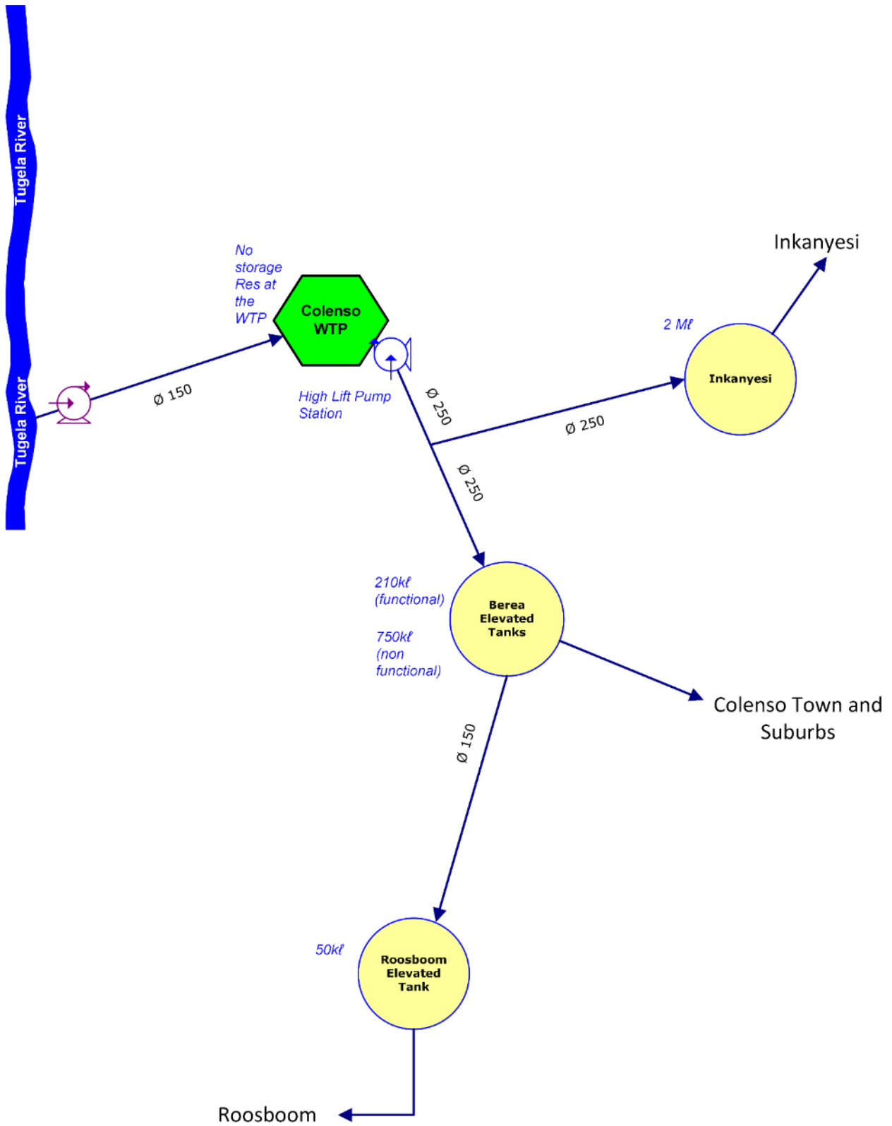
Figure 13.56 Colenso WTP Supply System Schematic (not to scale; uTDM Infrastructure)
