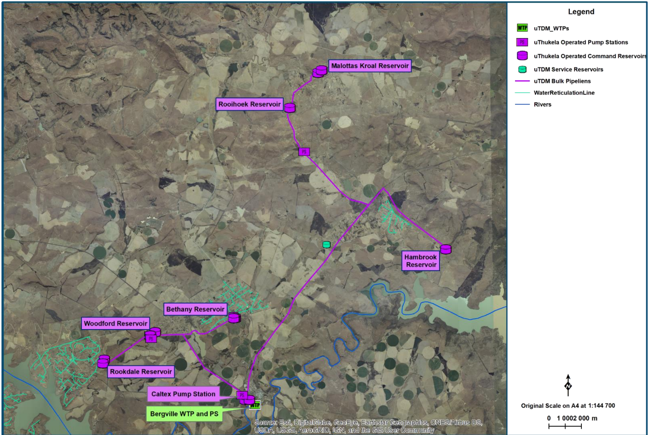
Figure 13.52 Bergville WTP Supply System Layout (NGI 2014; Umgeni Water 2020)
