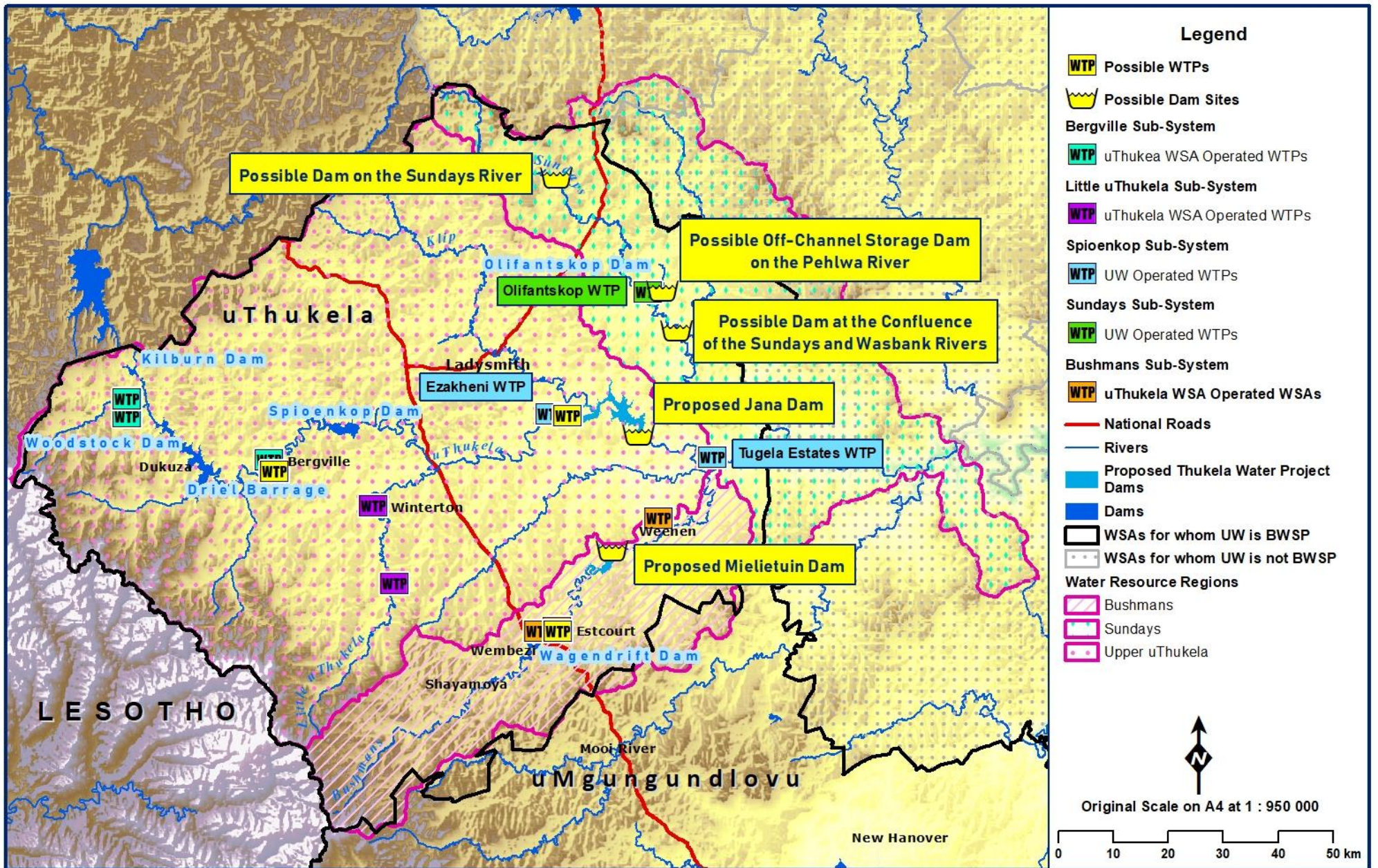
Figure 13.79 Possible water resource infrastructure options to be investigated (after DWA 2000 and DWA 2011, KZN DoT 2017, MDB 2016, Umgeni Water 2019, WR2012).
