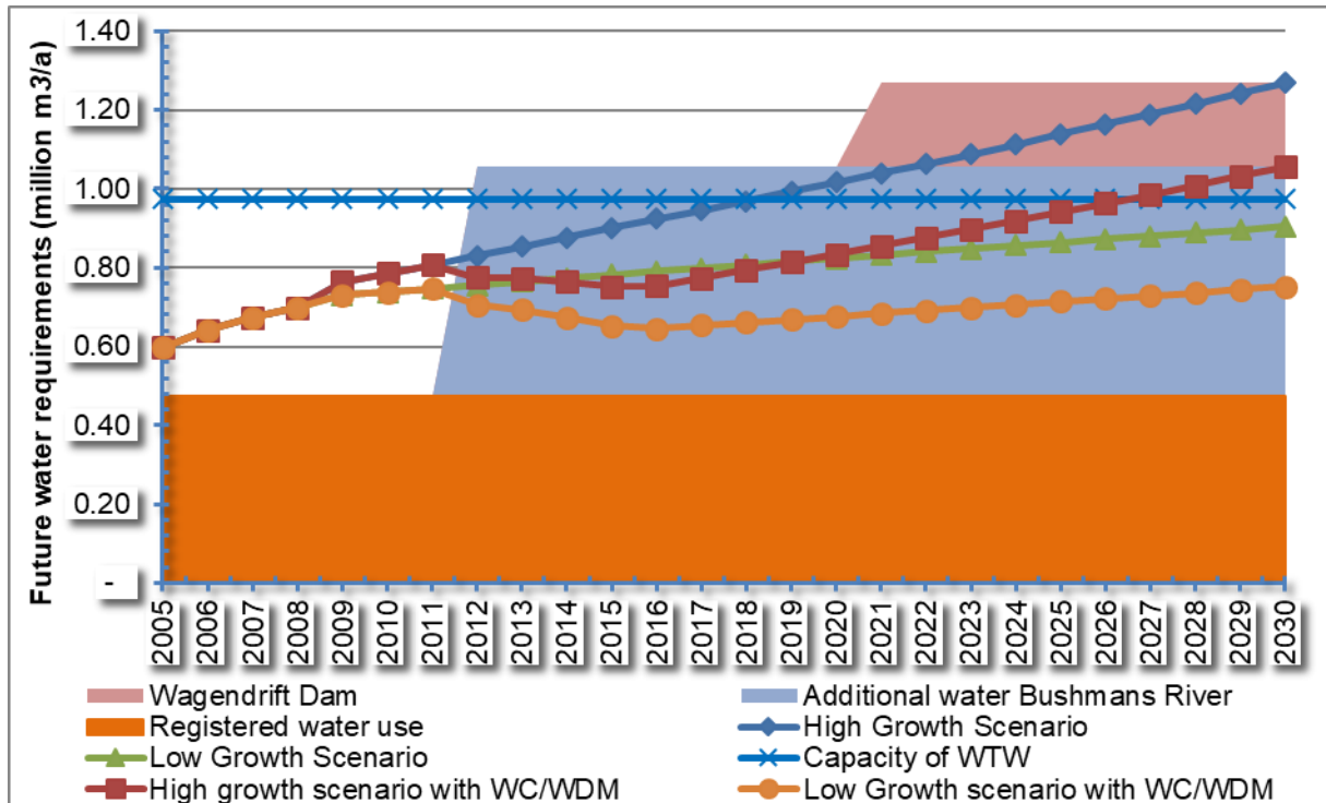
Figure 13.76 Water Reconciliation options to meet water requirements for Weenen Water Supply Scheme (DWS 2011: 32)
