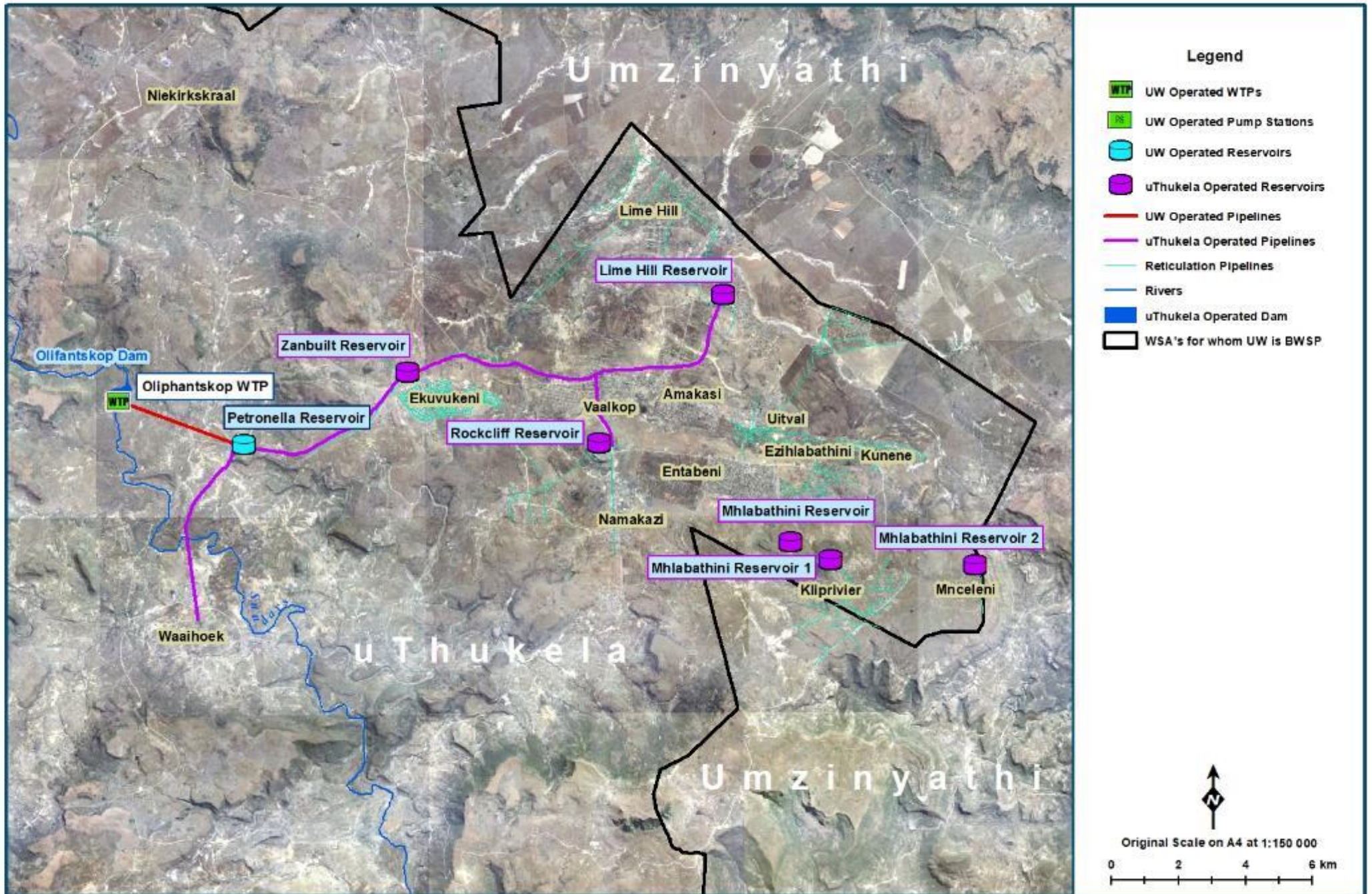
Figure 13.38 Olifantskop WTP Supply System layout (NGI 2014; Umgeni Water 2019).
