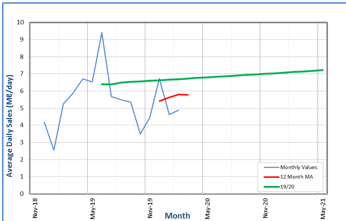
Figure 13.74 Water Demand from Olifantskop WTP
