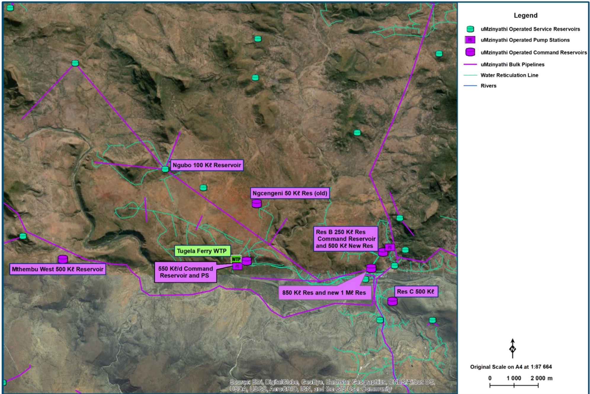
Figure 13.70 Tugela Ferry WTP Supply System Layout (NGI 2014; Umgeni Water 2020)
