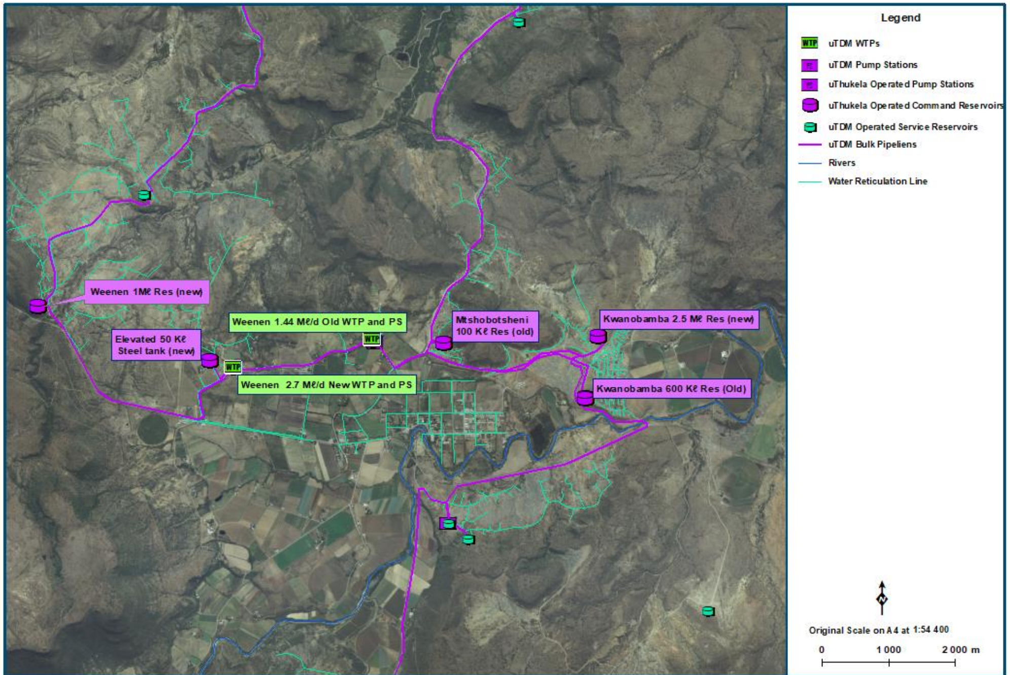
Figure 13.67 Weenen WTP Supply System Layout (NGI 2014; Umgeni Water 2020)
