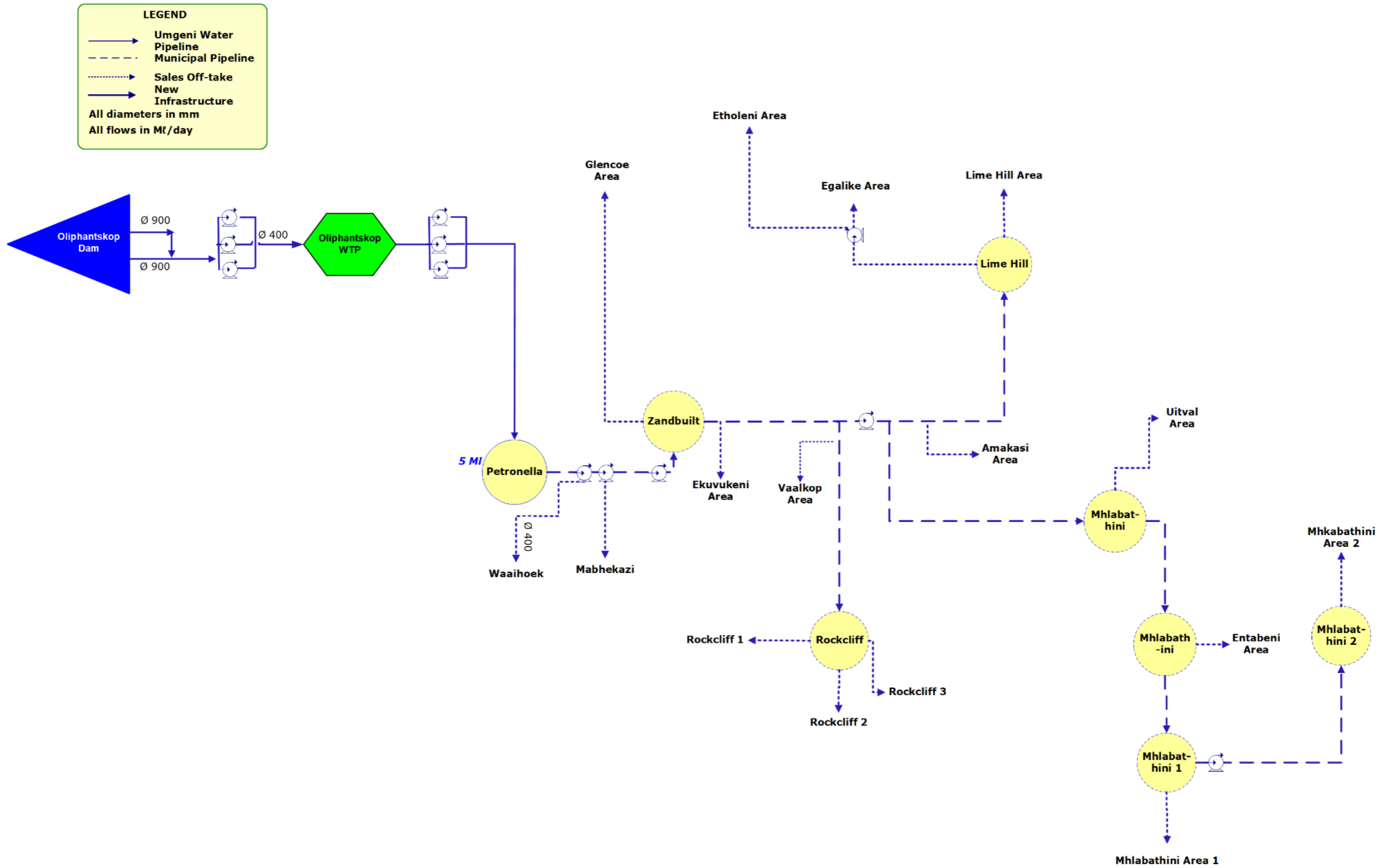
Figure 13.39 Oliphantskop WTP Supply System schematic.
