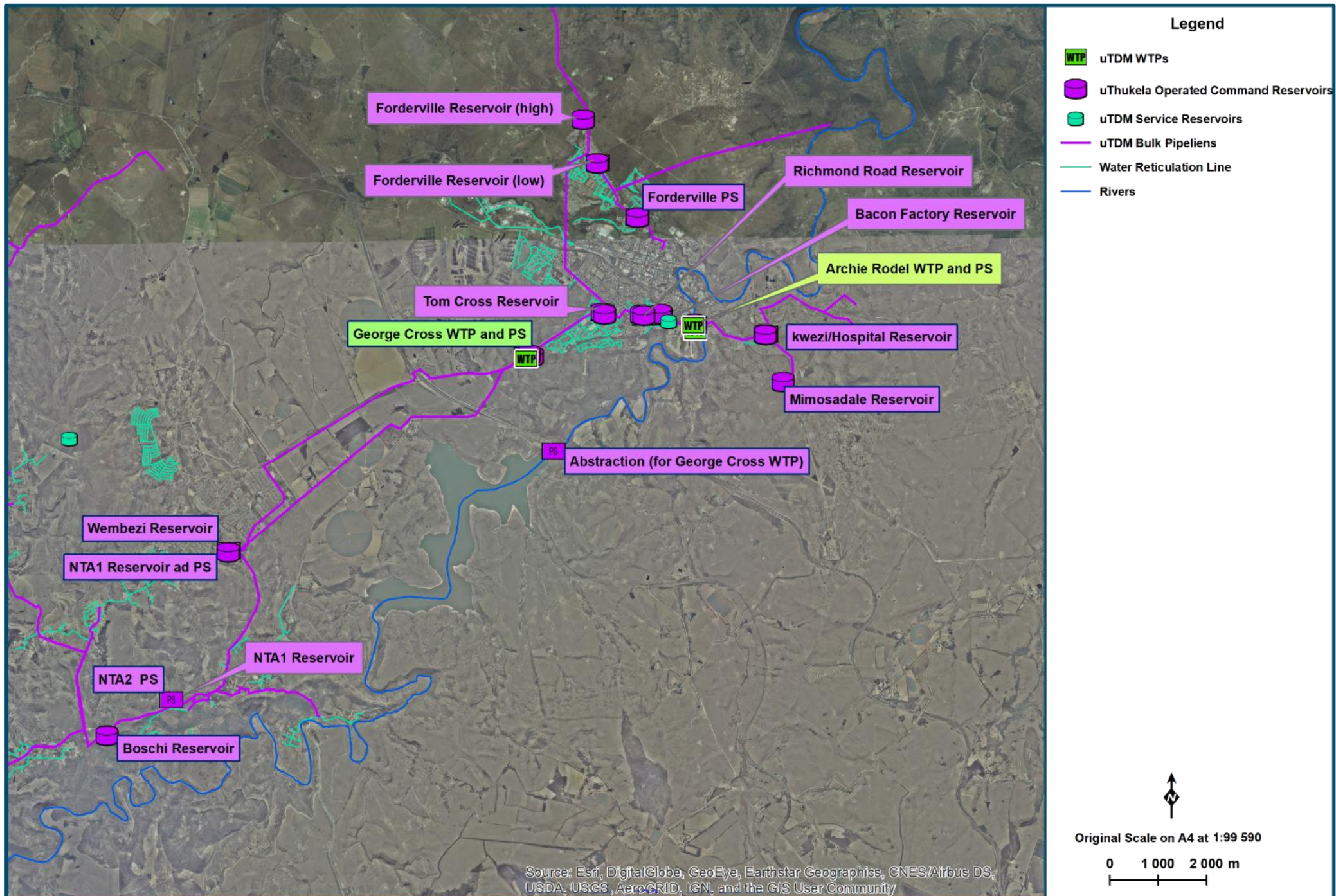
Figure 13.64 George Cross WTP (Estcourt) WTP Supply System Layout (NGI 2014; Umgeni Water 2020) (Note: this map also includes Archie Rodel WTP)
