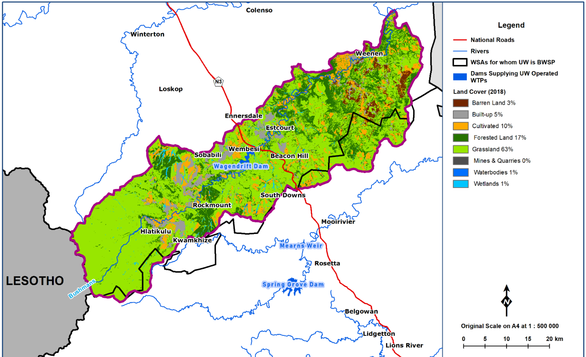
Figure 13.9 General layout of the Bushmans Region (DEA and GTI 2015, KZN DoT 2017, MDB 2016, Umgeni Water 2019).
