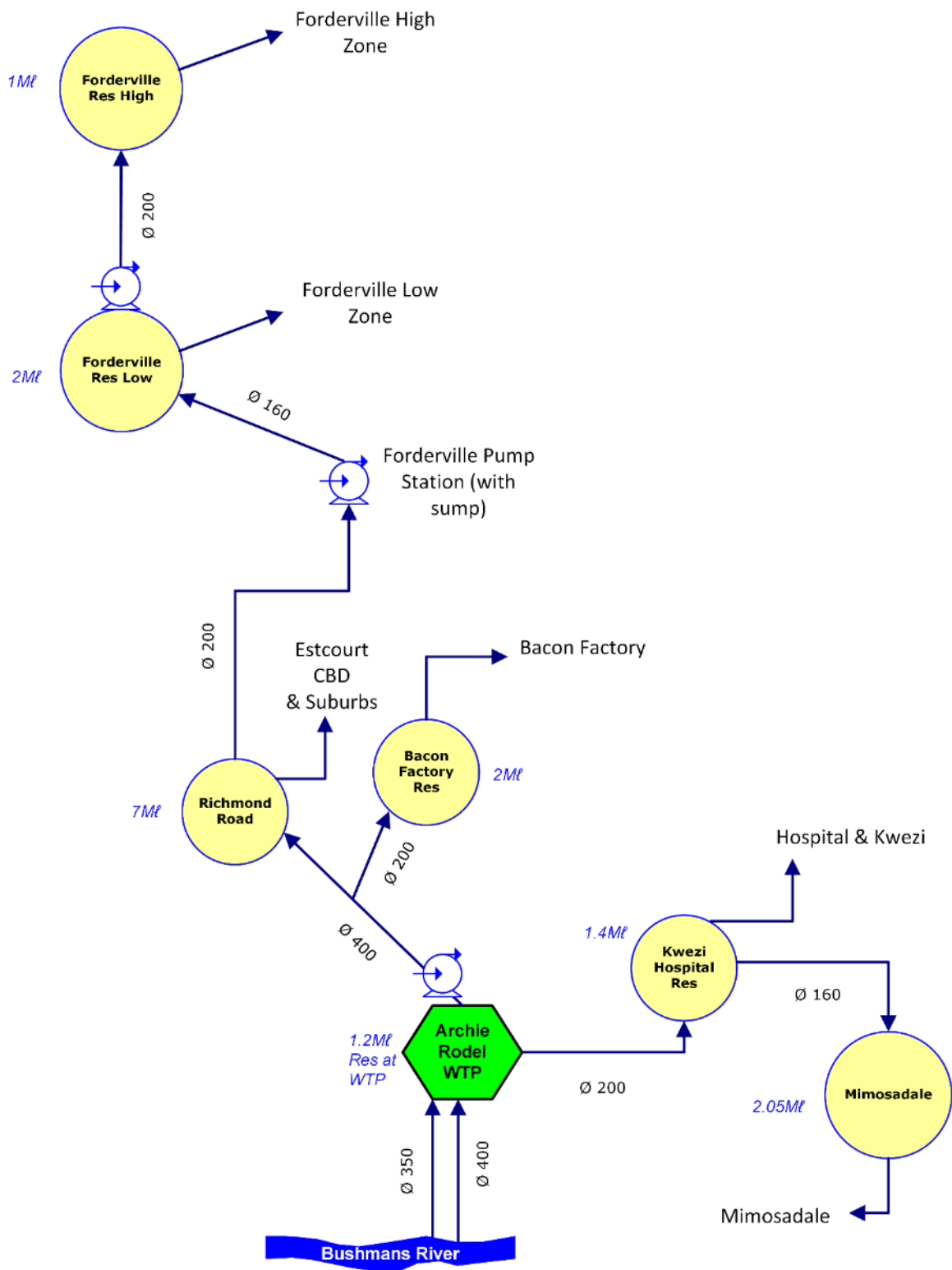
Figure 13.62 Archie Rodel WTP Supply System Schematic (not to scale; uTDM Infrastructure)
