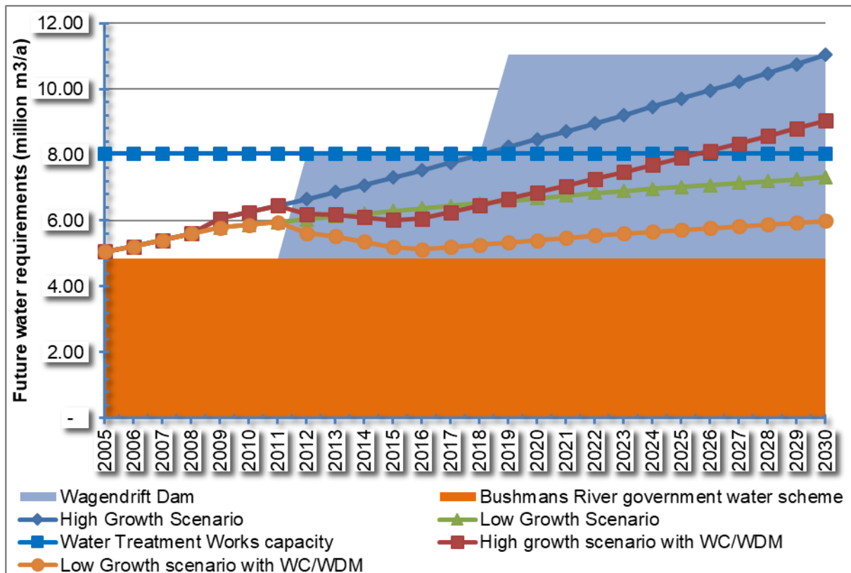
Figure 13.77 Water Reconciliation options to meet water requirements for Weenen Water Supply Scheme (DWS 2011: 35)
