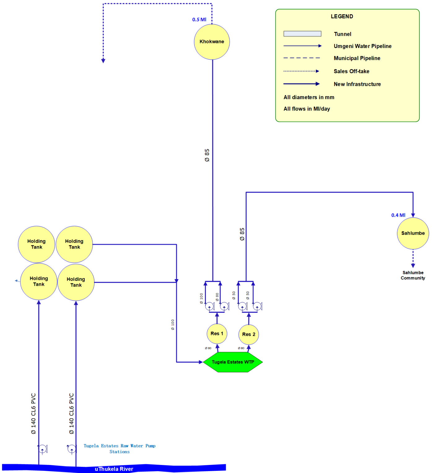
Figure 13.35 Tugela Estates WTP Supply System schematic.
