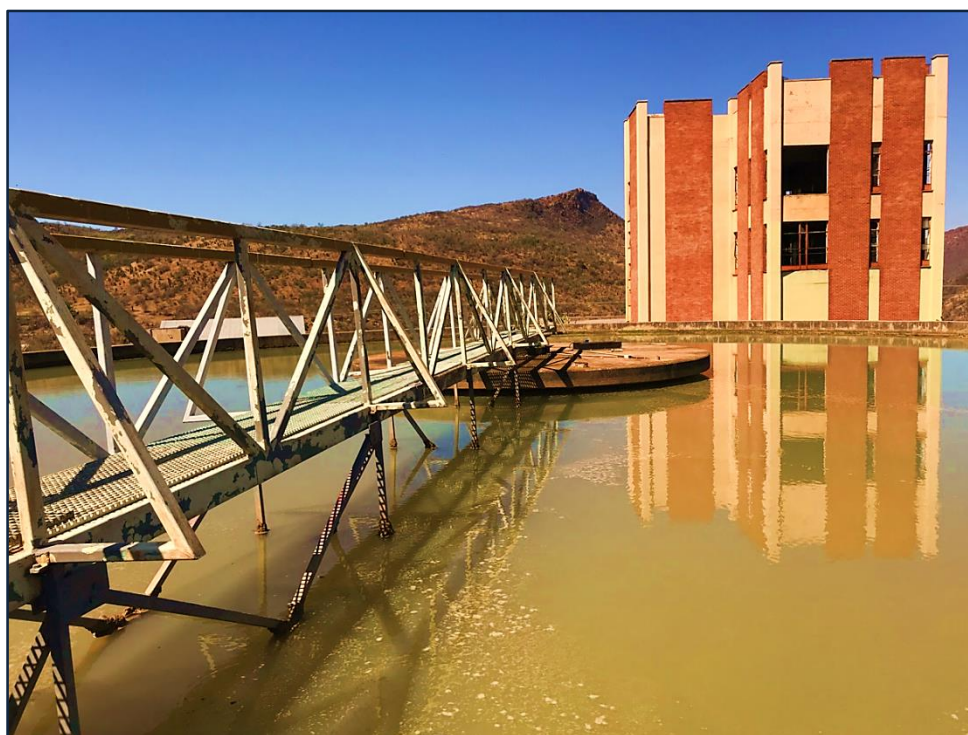
Figure 13.23 Ezakheni Water Treatment Plant (unknown date).
