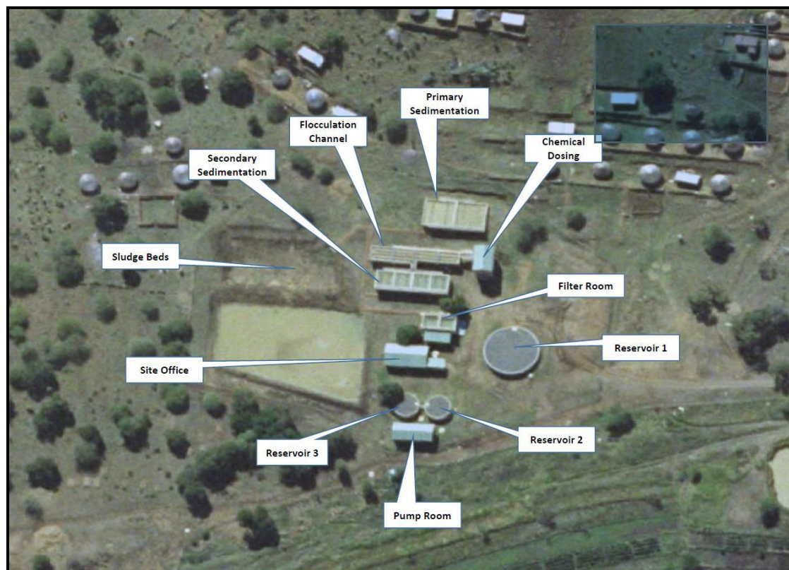
Figure 13.69 Overview of Tugela Ferry WTP, uMzinyathi DM O&M Manual (Dec2016)
