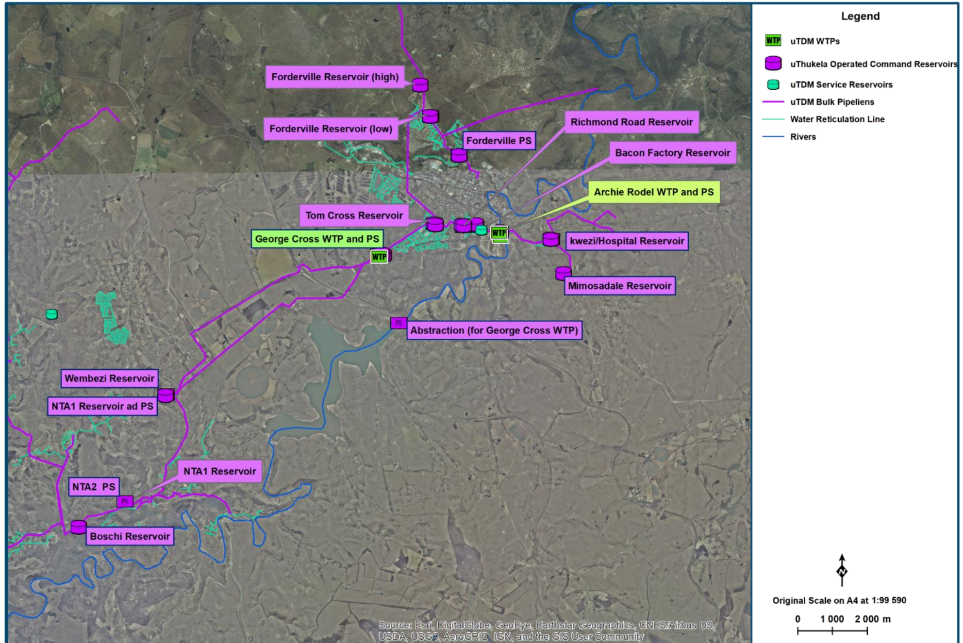
Figure 13.61 Archie Rodel (Estcourt) WTP Supply System Layout (NGI 2014; Umgeni Water 2020) (Note: this map also includes George Cross WTP)
