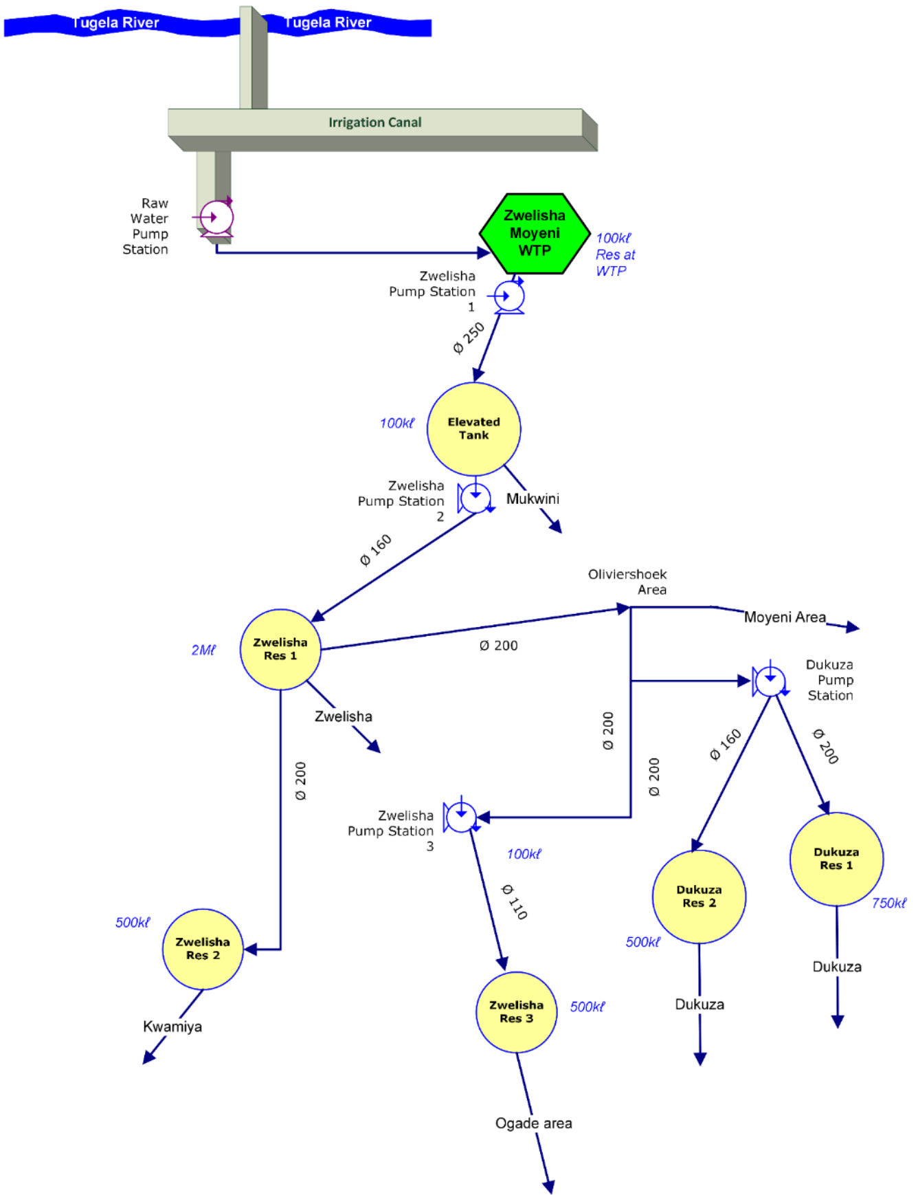
Figure 13.50 Zwelisha Moyeni WTP Supply System Schematic (not to scale; uTDM Infrastructure)
