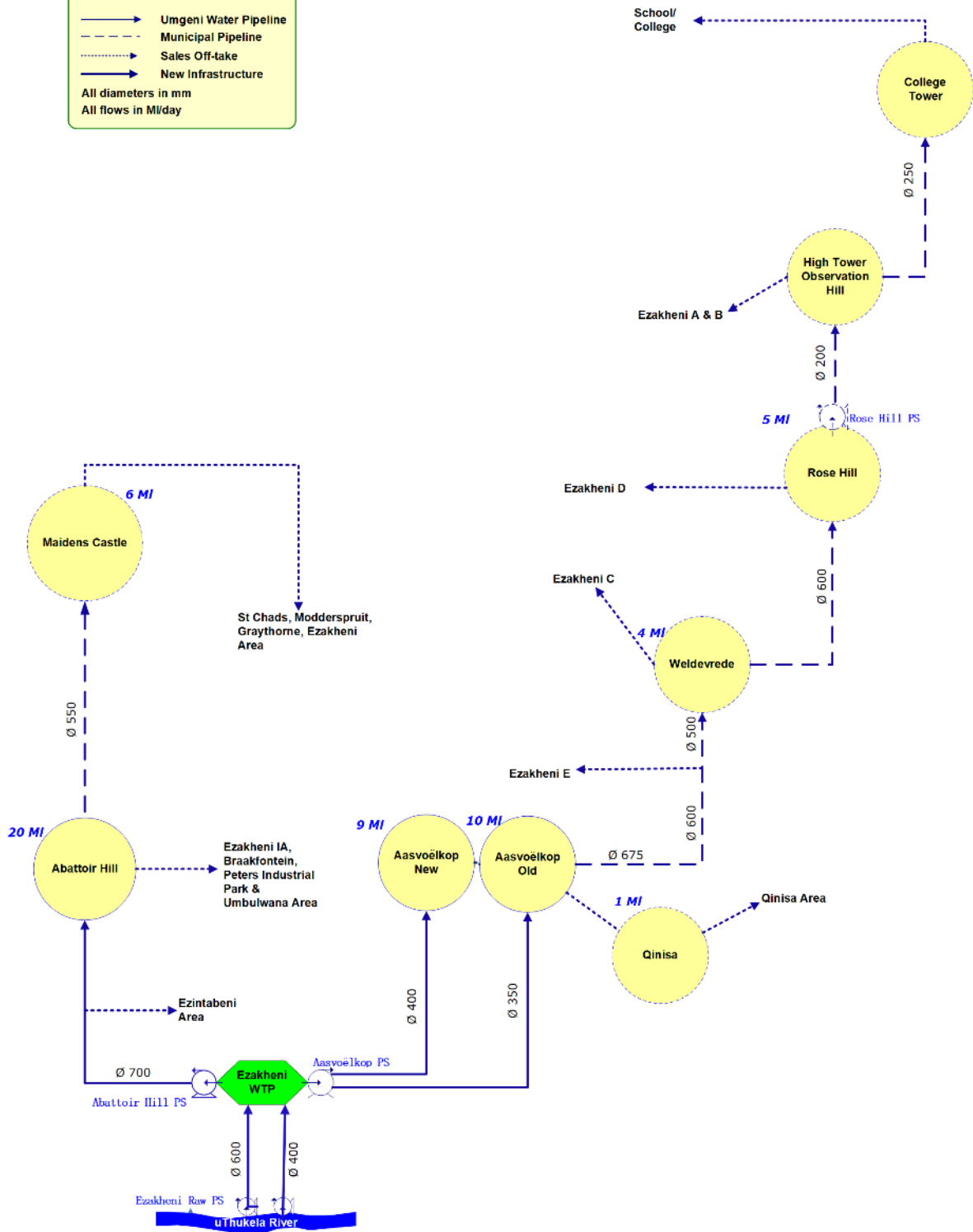
Figure 13.25 Ezakheni WTP Supply System schematic.
