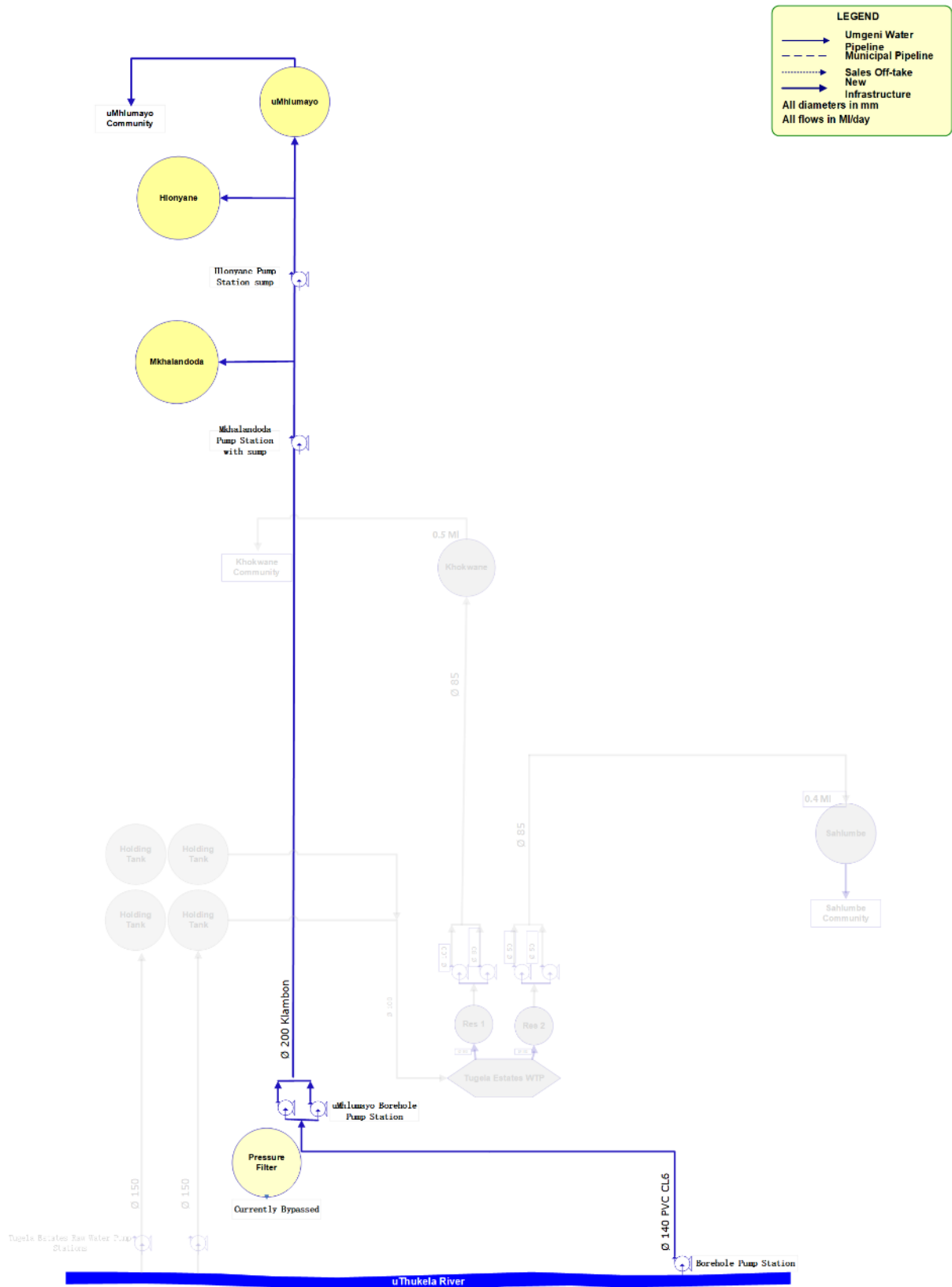
Figure 13.36 uMhlumayo Borehole Supply System schematic.
