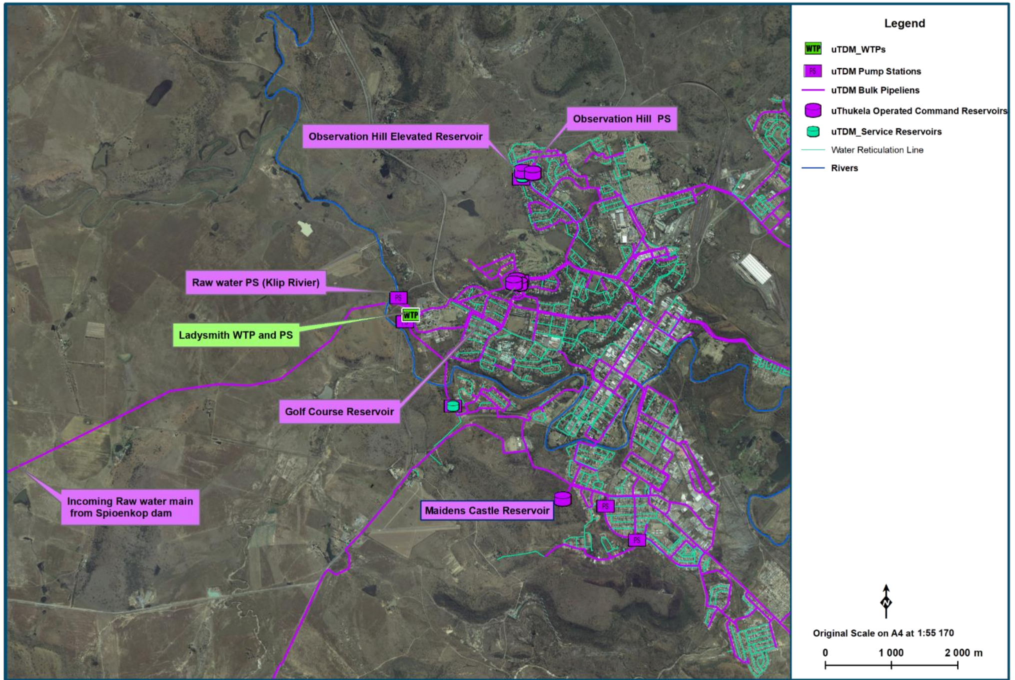
Figure 13.58 Ladysmith WTP Supply System Layout (NGI 2014; Umgeni Water)
