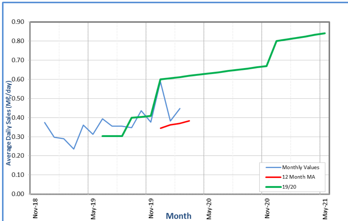
Figure 13.73 Water Demand from Tugela Estates WTP
