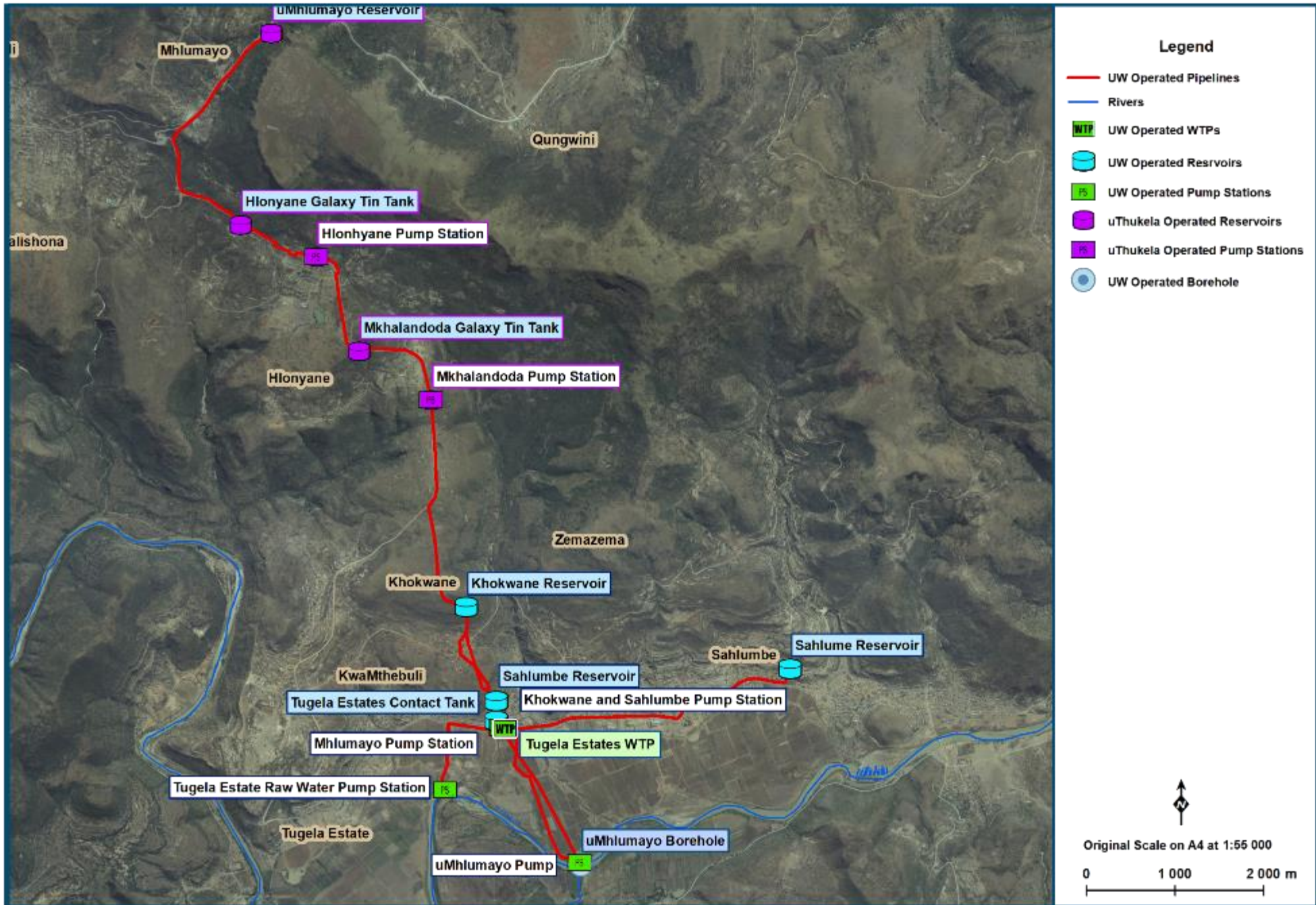
Figure 13.28 Tugela Estates WTP and uMhlumayo Borehole Supply System layout (NGI 2014; Umgeni Water 2019).
