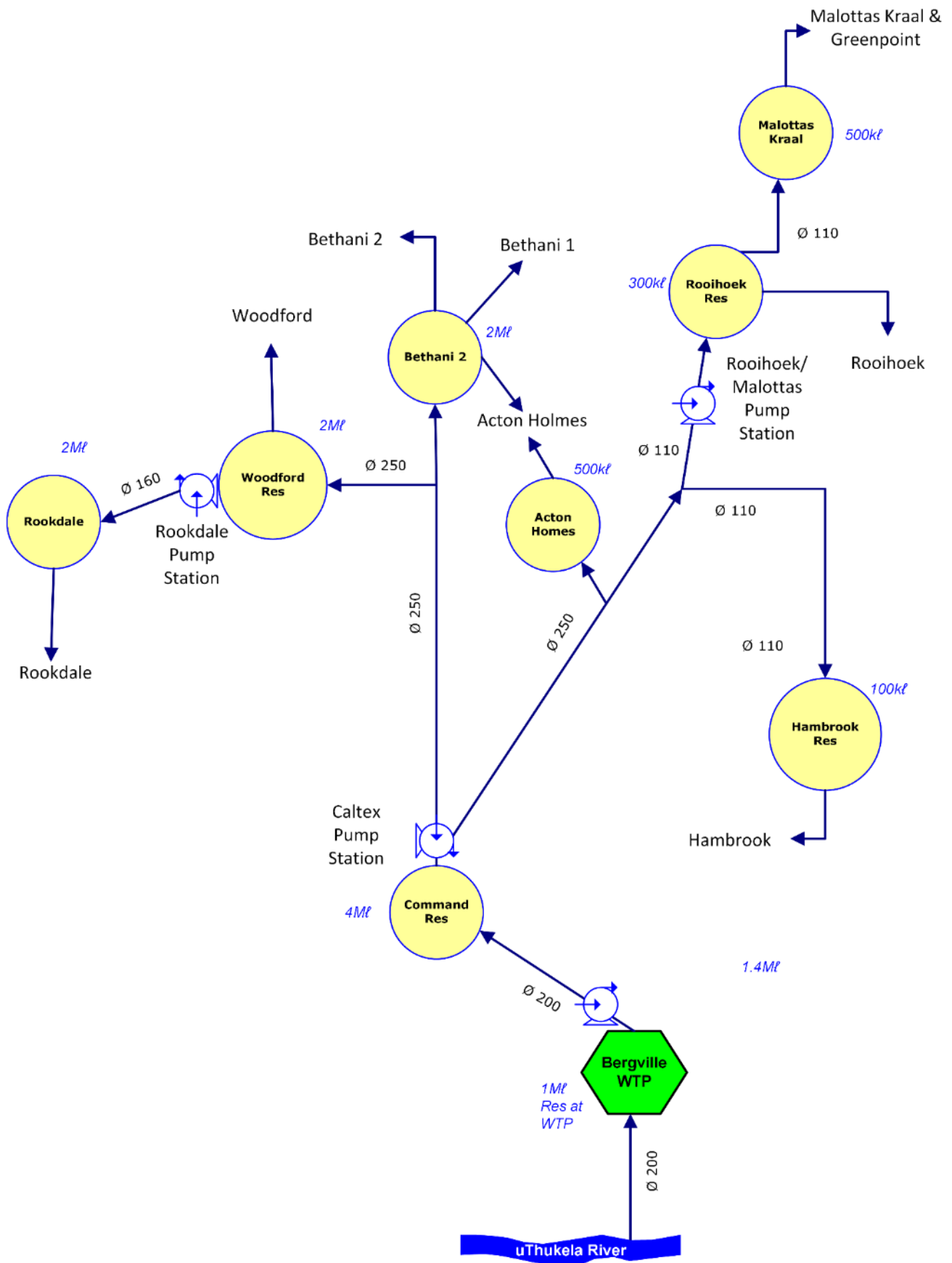
Figure 13.53 Bergville WTP Supply System Schematic (not to scale; uTDM Infrastructure)
