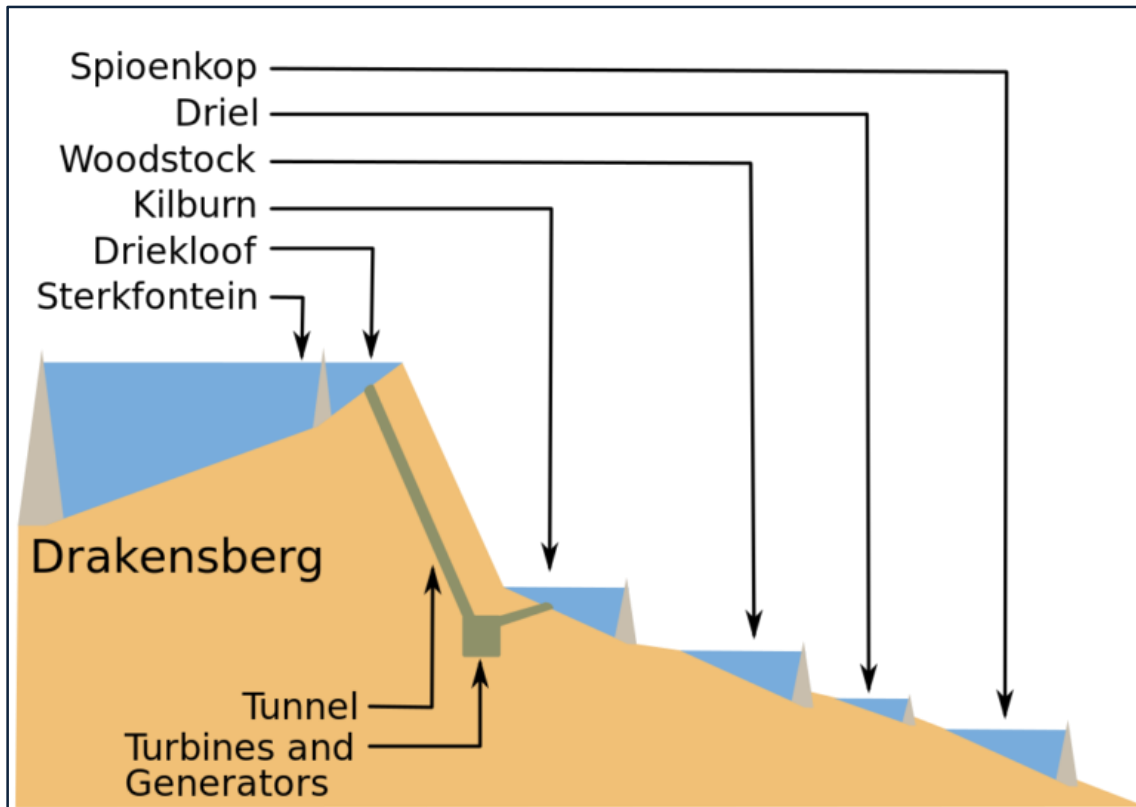
Figure 13.22 Longitudinal profile of the Thukela-Vaal Scheme and the Drakensberg Pumped Storage Scheme (Ladysmith Gazette 2017: website 22 ).
