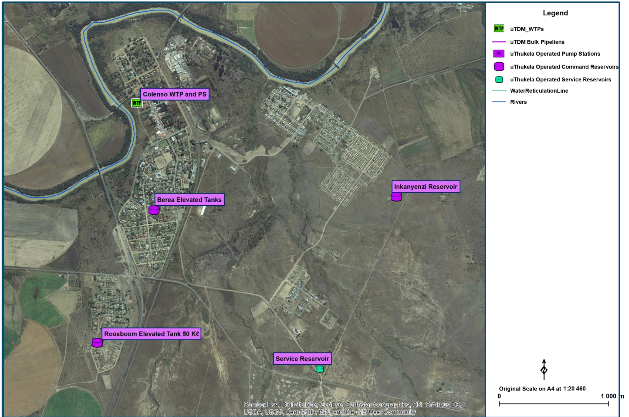
Figure 13.55 Colenso WTP Supply System Layout (NGI 2014; Umgeni Water 2020)
