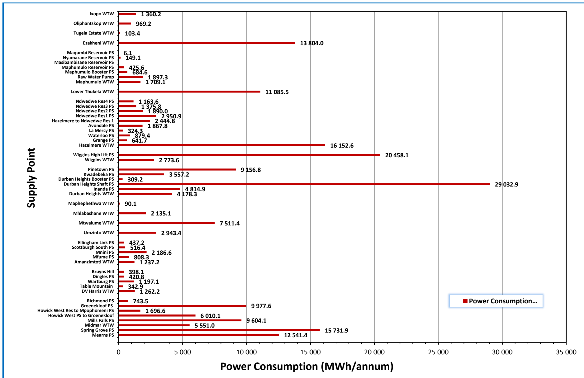
Figure 5.3 Annual Power Usage Comparison Umgeni Water Installations.
