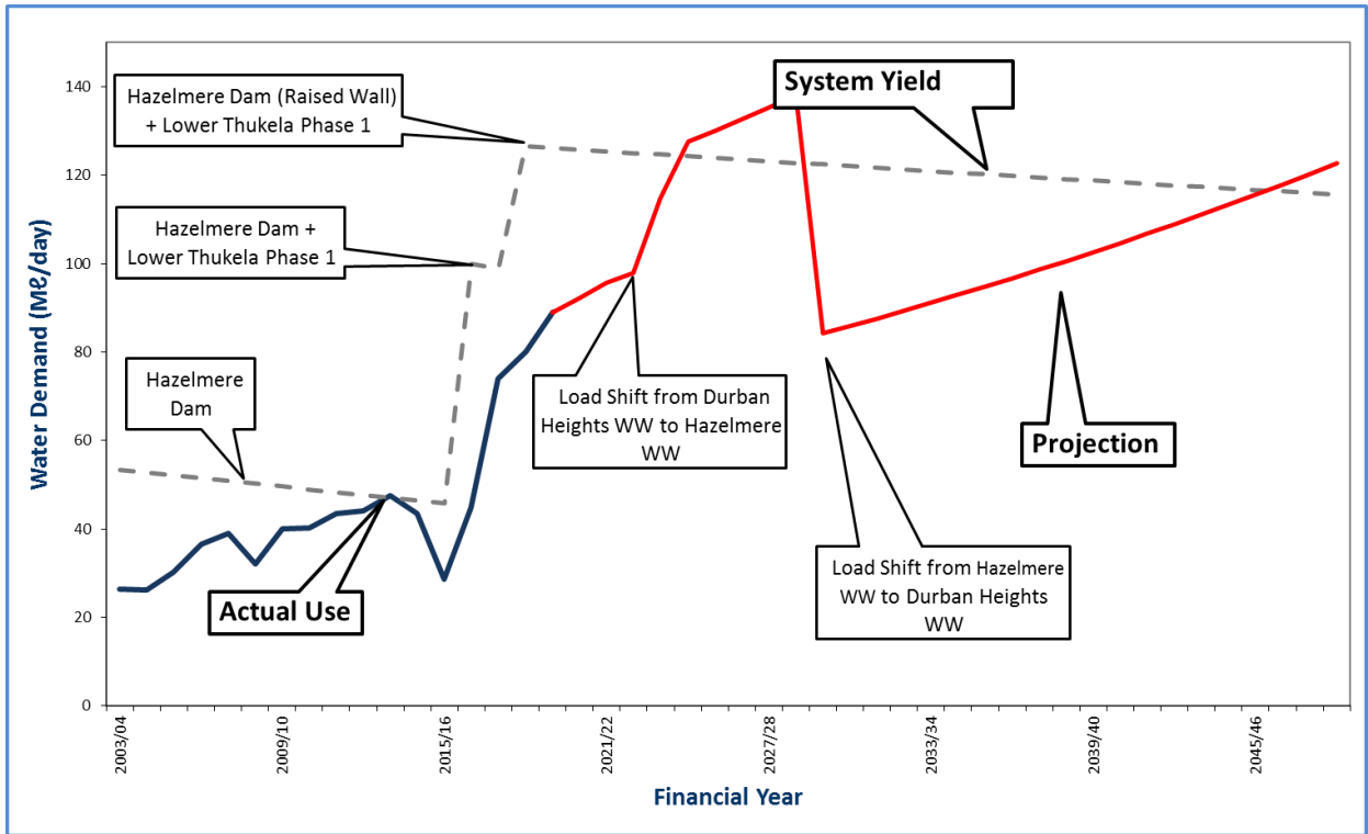
Figure 2.73 North Coast Supply System – Existing Water Balance
