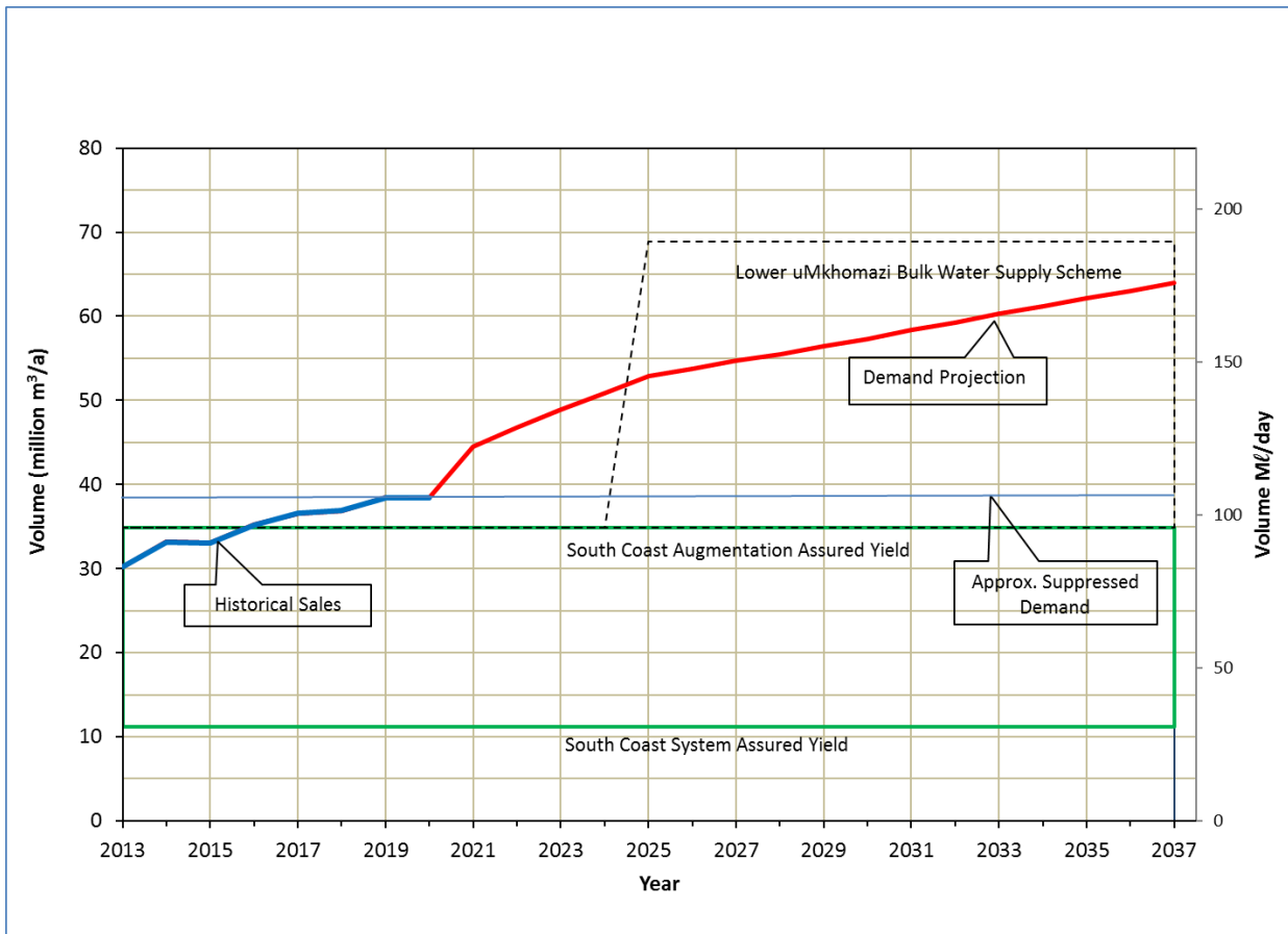
Figure 2.74 South Coast Supply System – Existing Water Balance
