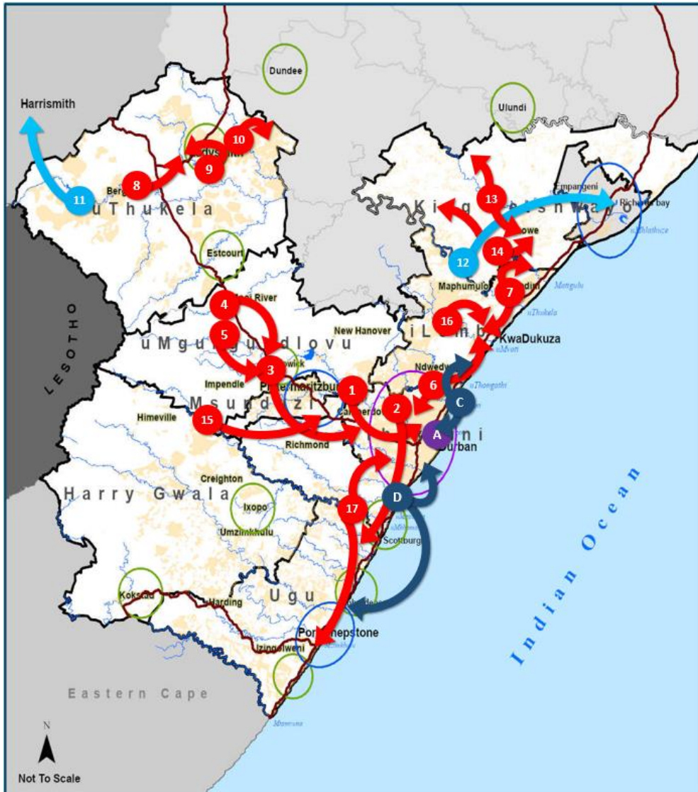
Figure 2.75 Future bulk water supply strategy.
