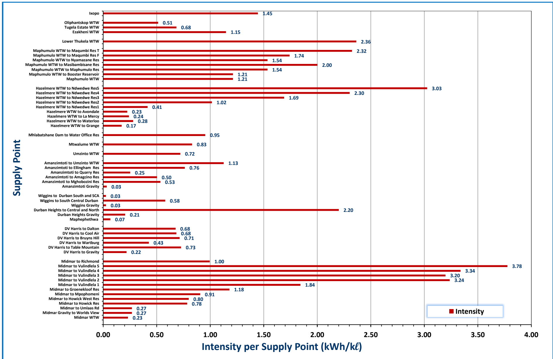
Figure 5.5 Annual Energy Intensity per Supply Point.
