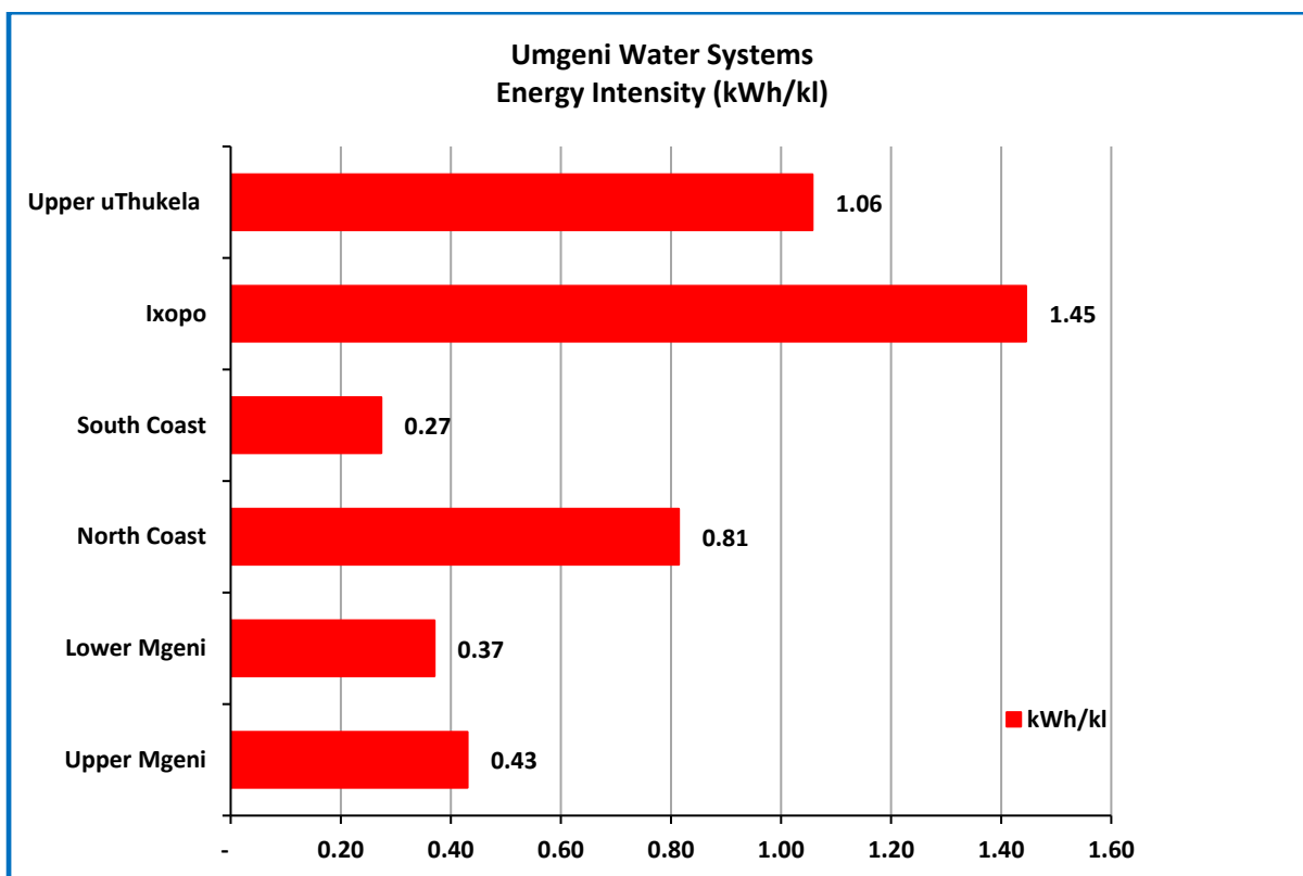
Figure 5.2 Energy requirement to supply water in Umgeni Water Systems 2019/20.
