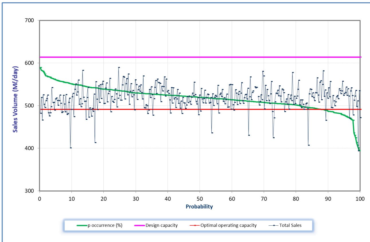
Figure 7.43 Analysis of historical production at Durban Heights WTP from November 2019 to October 2020.
