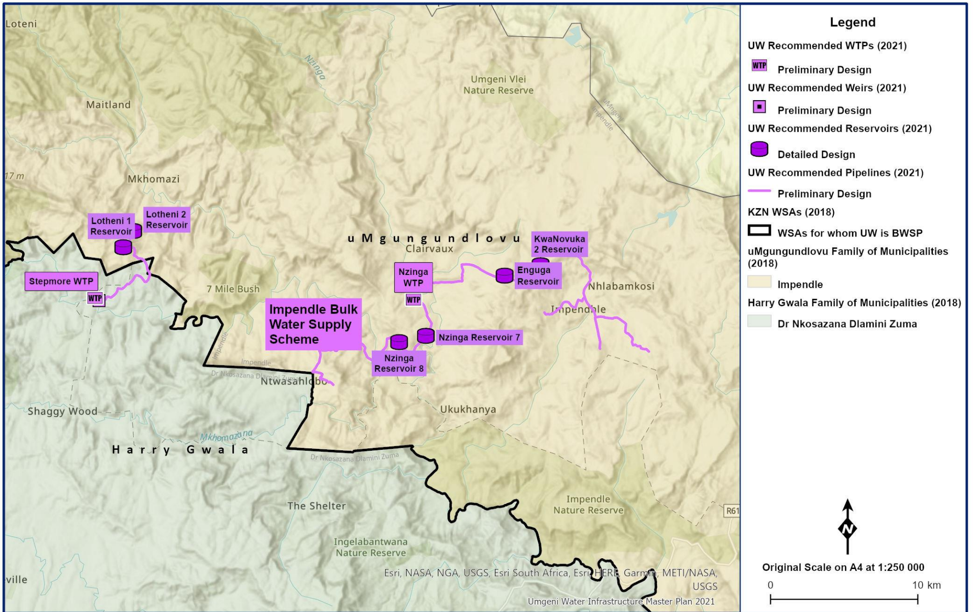
Figure 7.63 General layout of the Impendle Project Areas.
