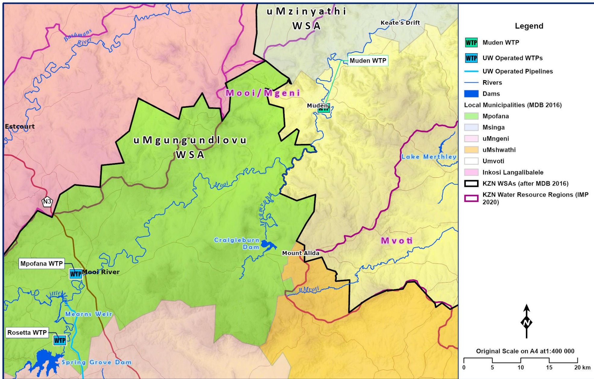
Figure 7.88 Muden WTP supply system.
