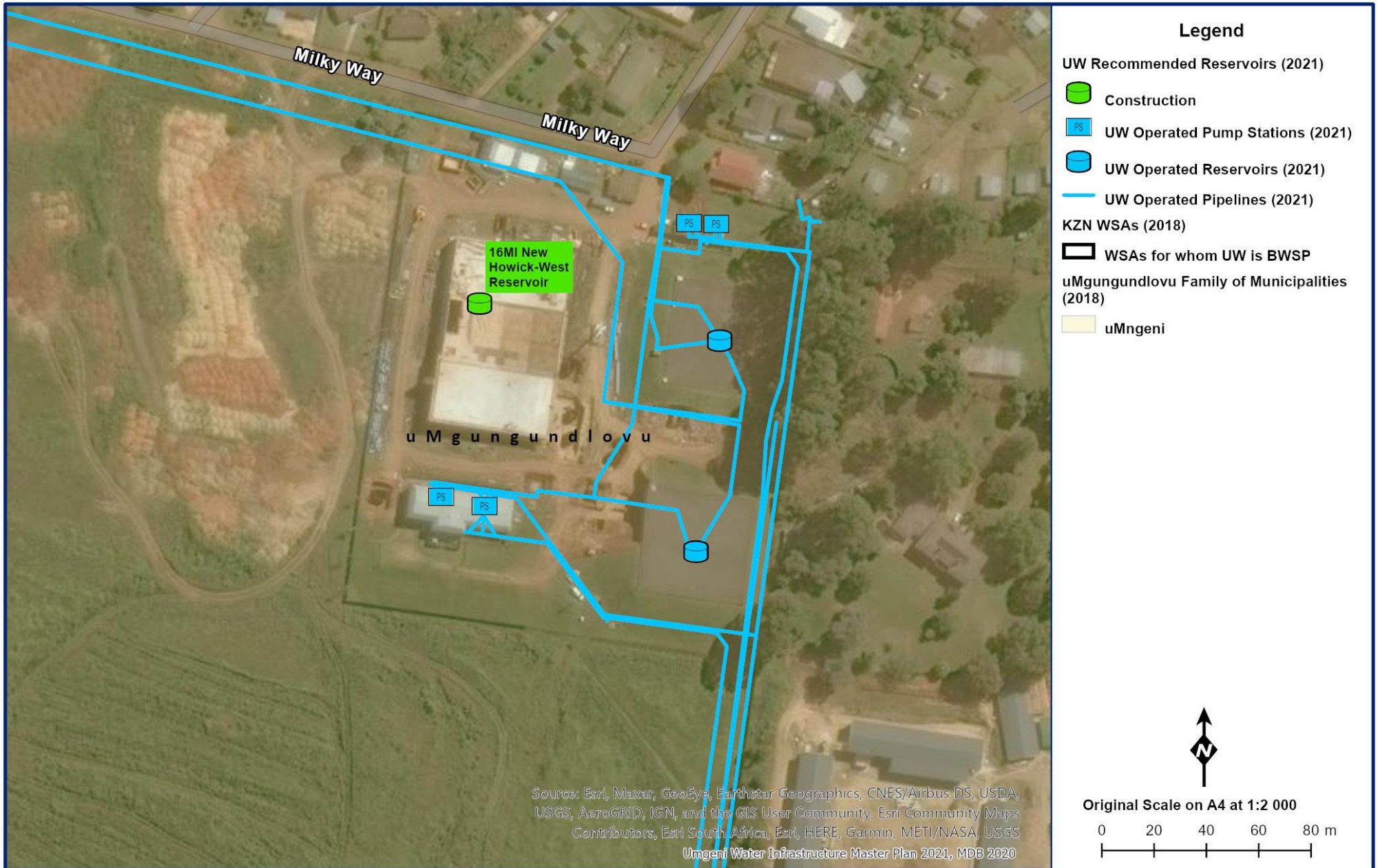
Figure 7.67 General layout of the proposed Howick-West Reservoir.
