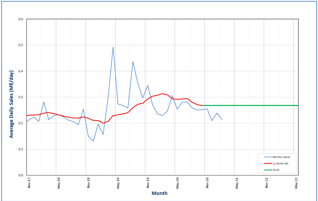
Figure 7.87 Water demand from Rosetta WTP.
