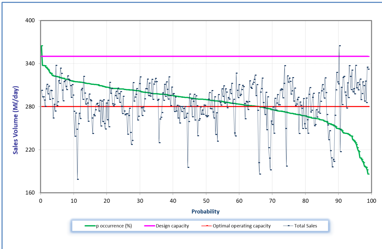
Figure 7.46 Analysis of historical production at Wiggins WTP from November 2019 to October 2020.
