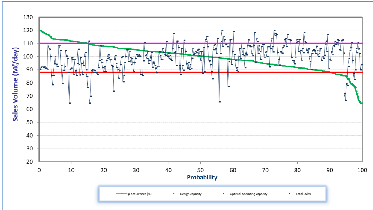
Figure 7.42 Analysis of historical production at D.V. Harris WTP (November 2019 to October 2020).
