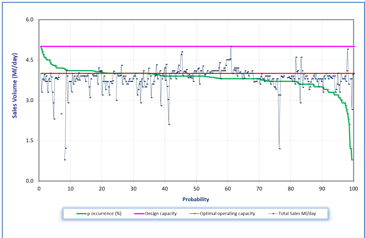
Figure 7.49 Analysis of historical production at Maphephethwa WTP from November 2019 to October 2020.
