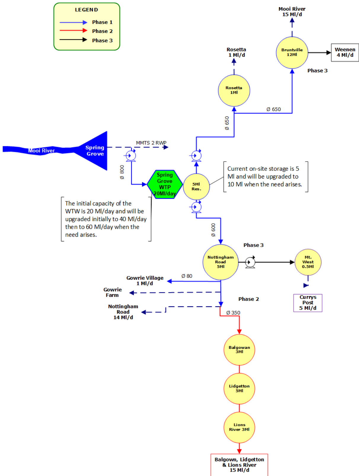
Figure 7.65 Schematic of Greater Mpofana BWSS.
