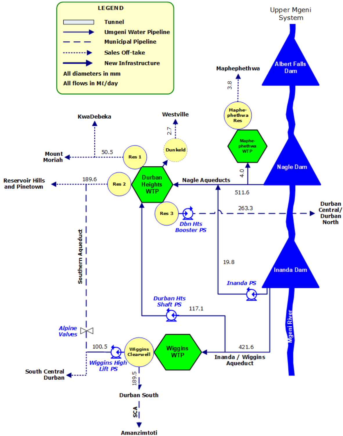
Figure 7.59 Schematic of the Lower Mgeni System.
