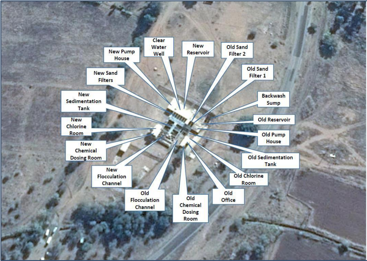
Figure 7.90 Aerial view of the Mudén WTP (Google Earth 2018).
