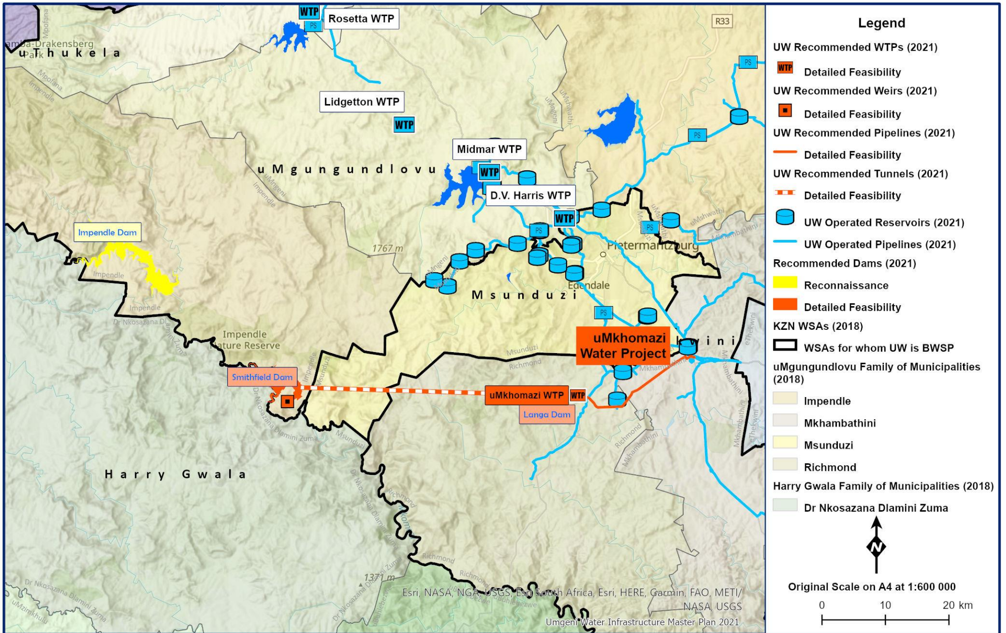
Figure 7.60 uMkhomazi Water Project.
