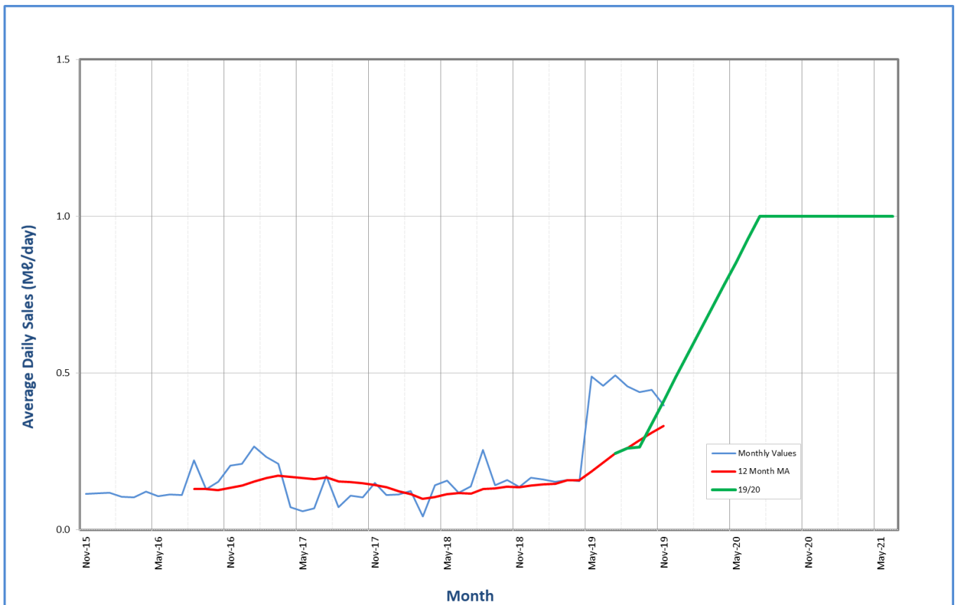
Figure 7.78 Water demand from Lidgetton WTP.
