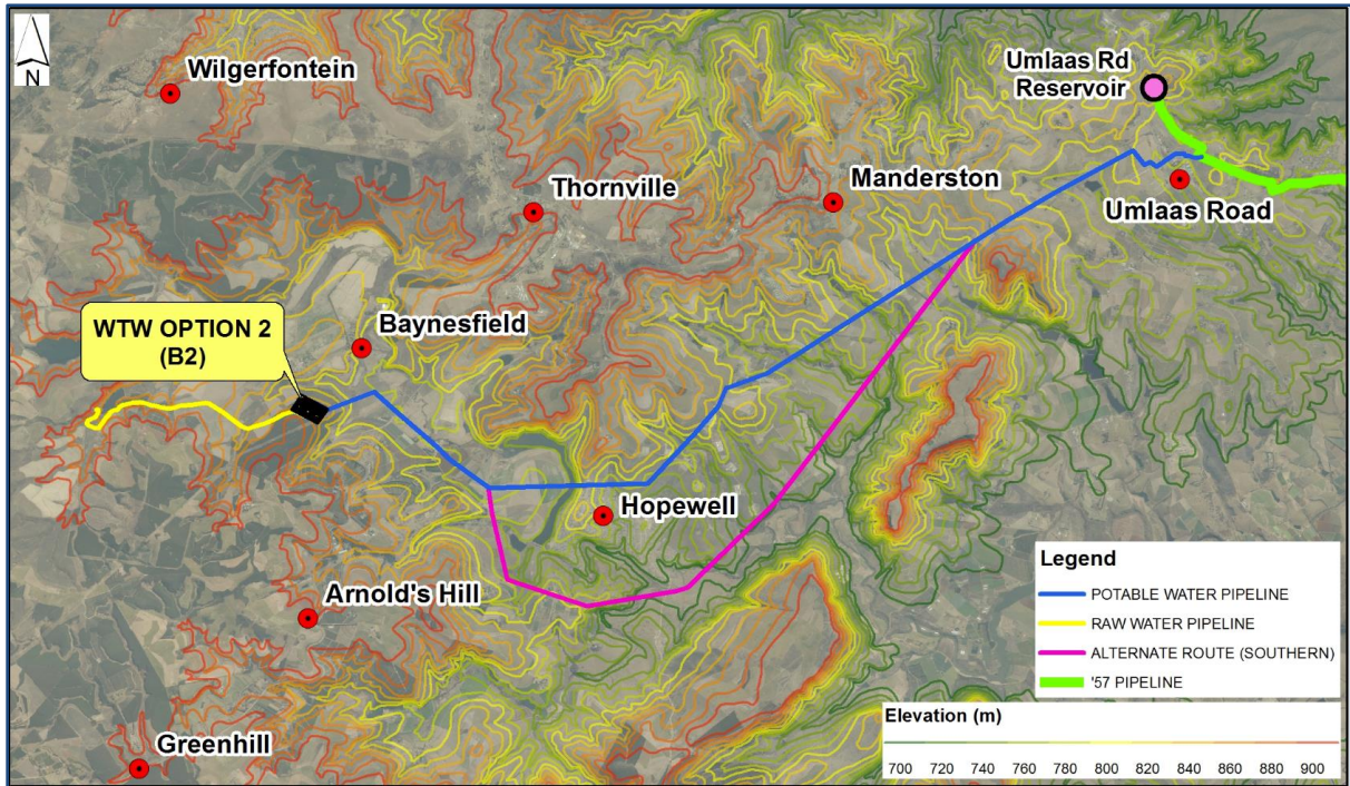
Figure 7.62 Layout of pipeline.
