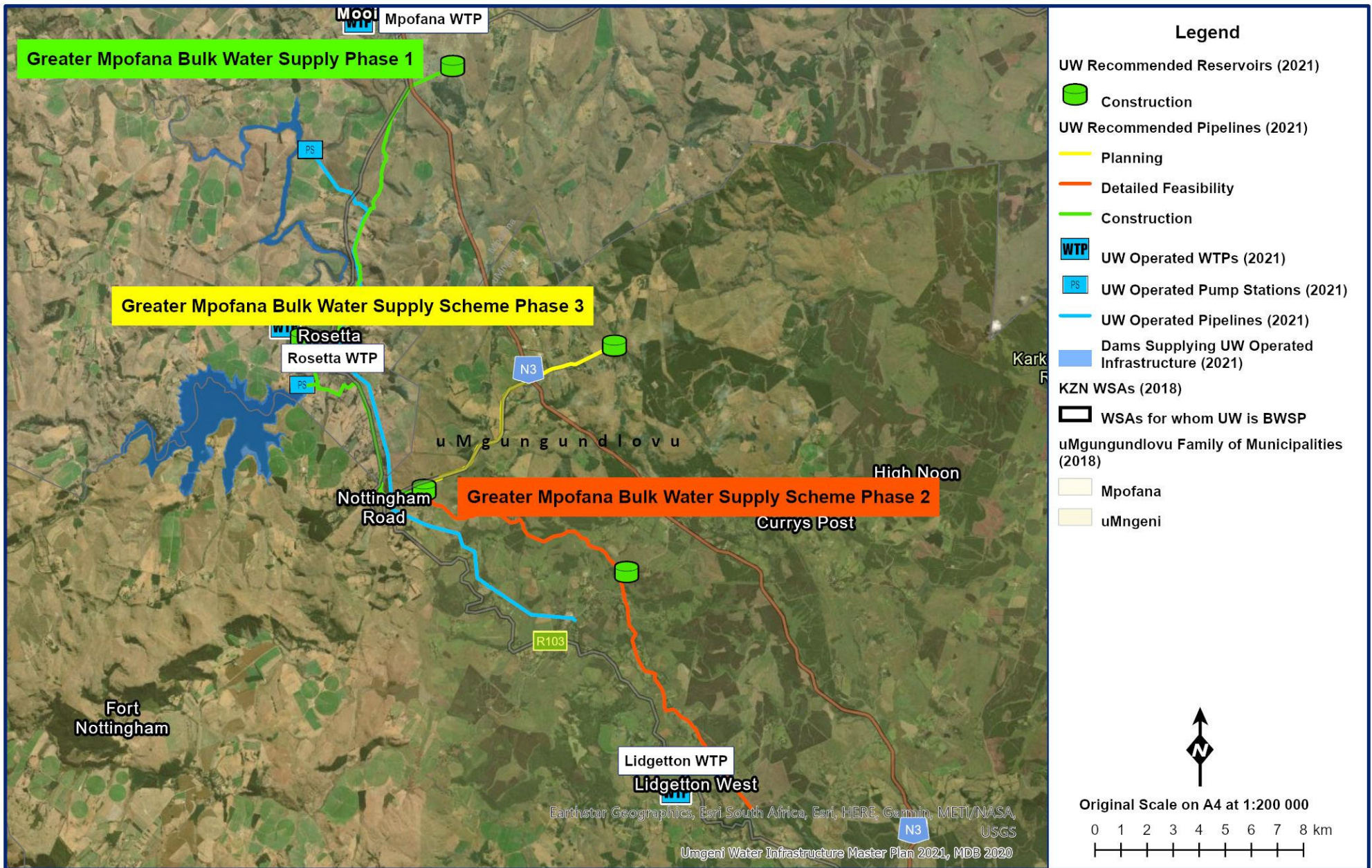
Figure 7.64 Greater Mpofana Bulk Water Supply Scheme.
