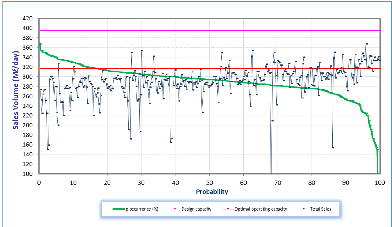
Figure 7.40 Analysis of historical production at Midmar WTP (November 2019 to October 2020).
