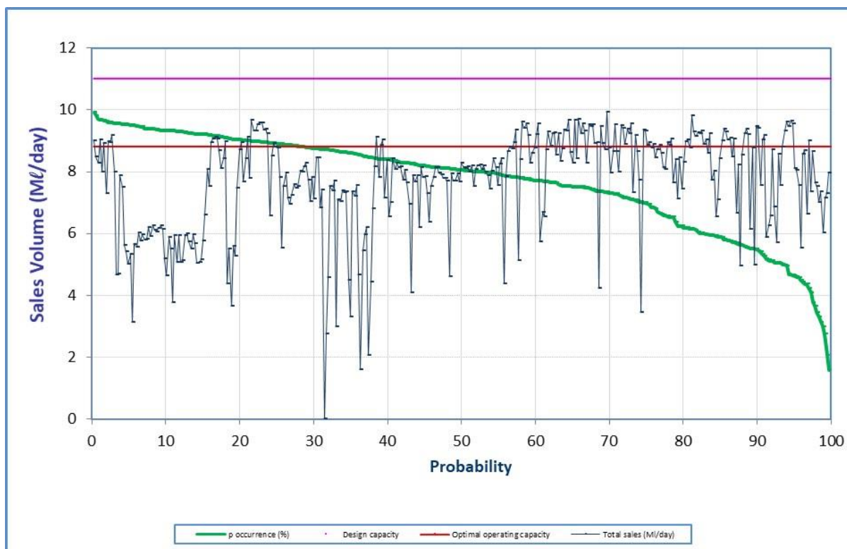
Figure 12.32 Analysis of historical production at Maphumulo WTP (November 2019 to October 2020).
