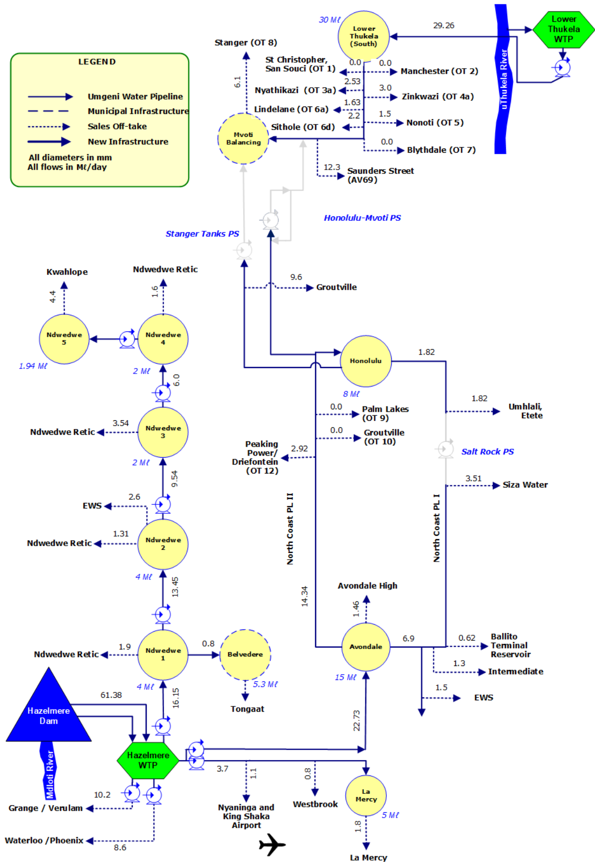
Figure 12.33 Demand on the North Coast Supply System as at October 2020.
