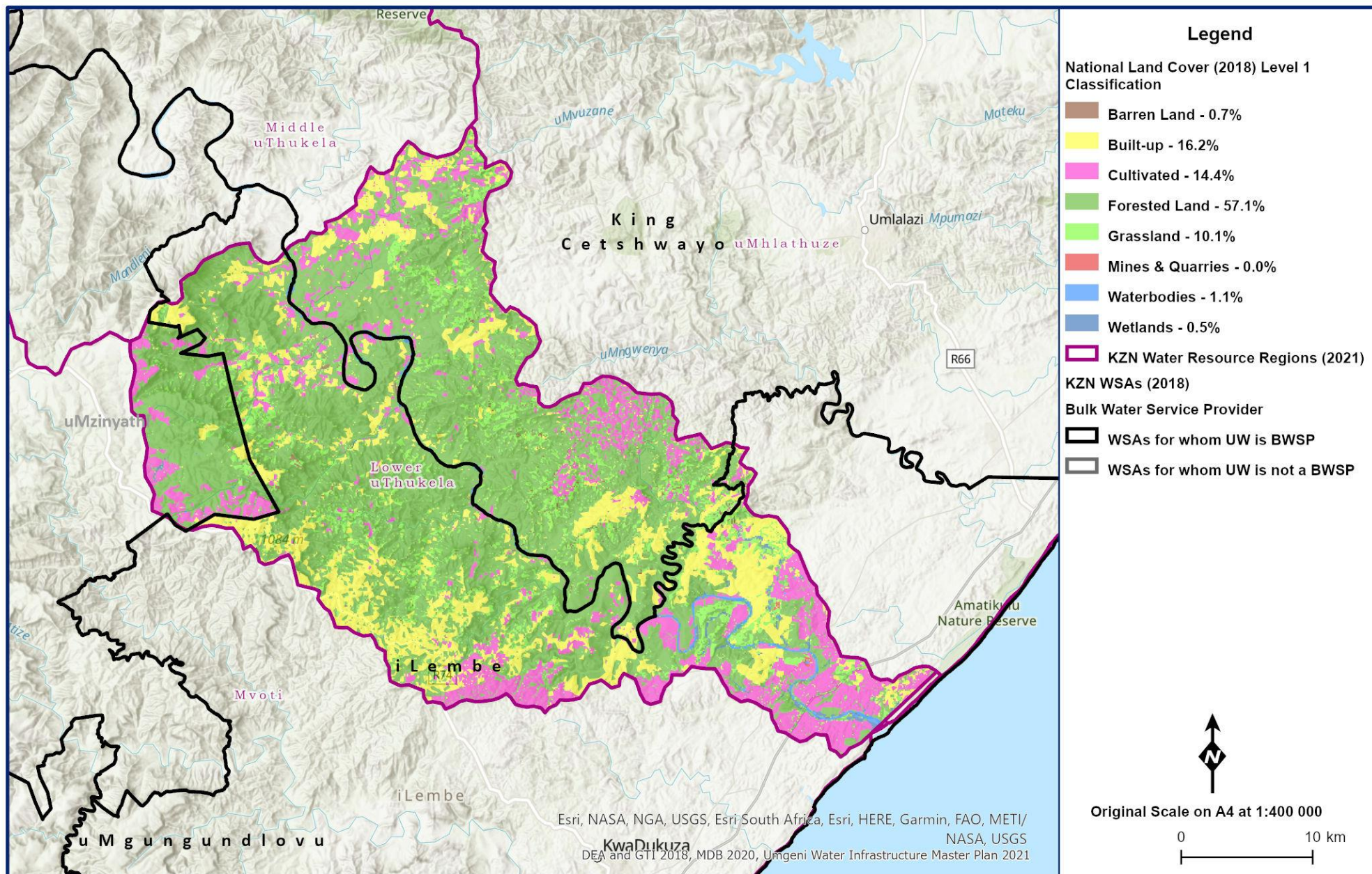
Figure 12.2 General layout of the Lower uThukela Region (DEA and GTI 2018; MDB 2020; Umgeni Water 2021; WR2012).
