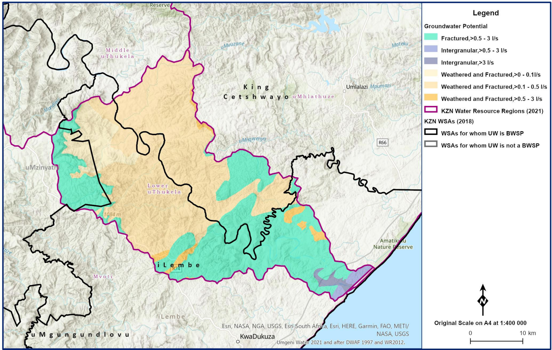
Figure 12.3 Groundwater potential in the uThukela Region (MDB 2018; Umgeni Water 2021; after DWAF 1997 and WR2012).
