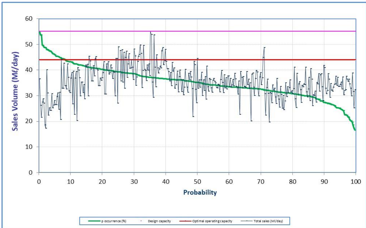
Figure 12.29 Water Demand from Lower Thukela WTP
