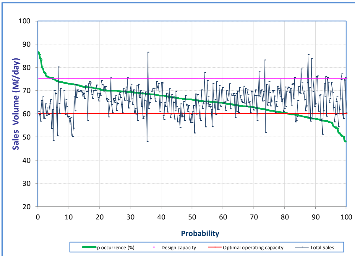
Figure 12.28 Analysis of historical production at Hazelmere WTP (November 2019 to October 2020).
